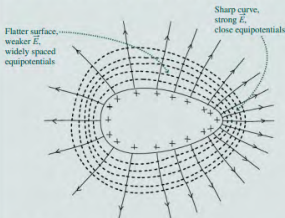
FIGURE 22.20 Equipotentials and field of a charged conductor.
