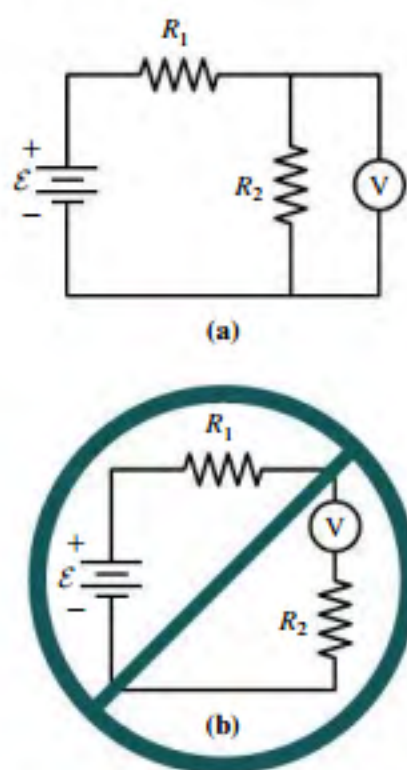
FIGURE 25.14 Correct (a) and incorrect (b) ways to connect a voltmeter for measuring the voltage across R_2 .
