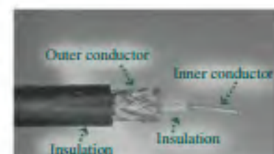
FIGURE 21.38 A coaxial cable (Passage Problems 76–79)
