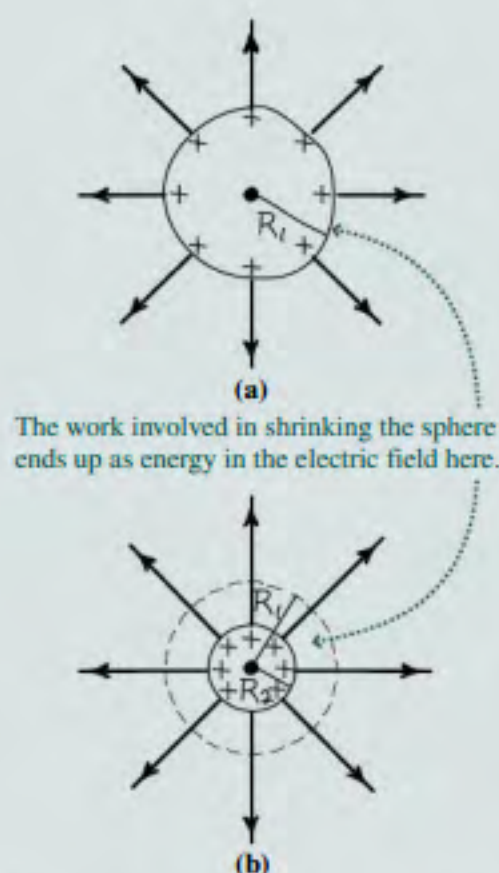
FIGURE 23.10 (a) A charged sphere and its electric field. (b) Shrinking the sphere creates field and energy in the region R_2 < r < R_1 .
