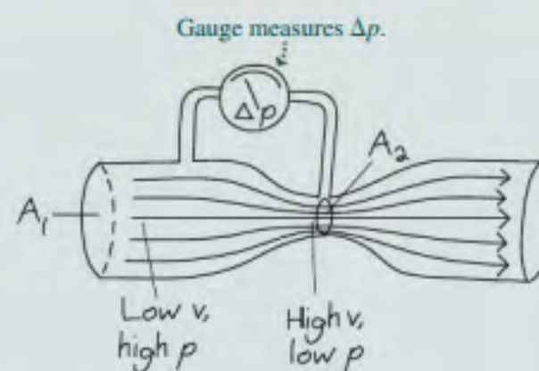
FIGURE 15.15 Our sketch of a venturi flowmeter.
