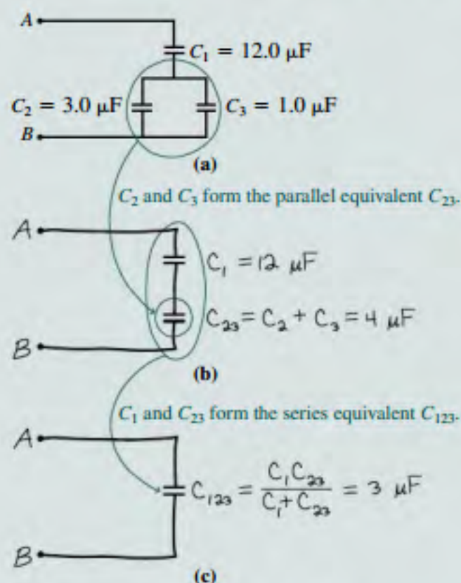
FIGURE 23.9 Finding the equivalent capacitance.
