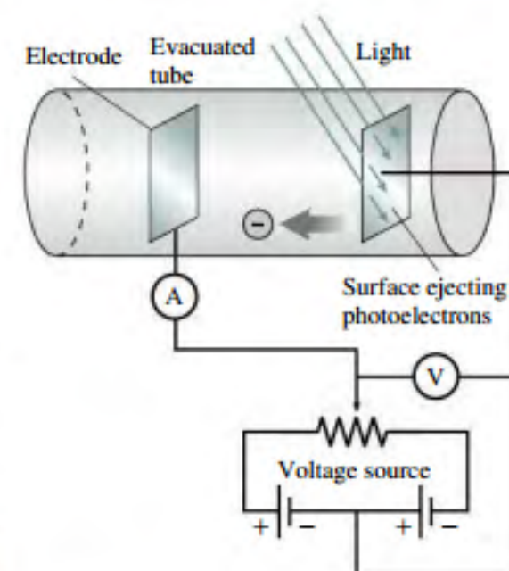
FIGURE 34.5 Apparatus for studying the photoelectric effect.
