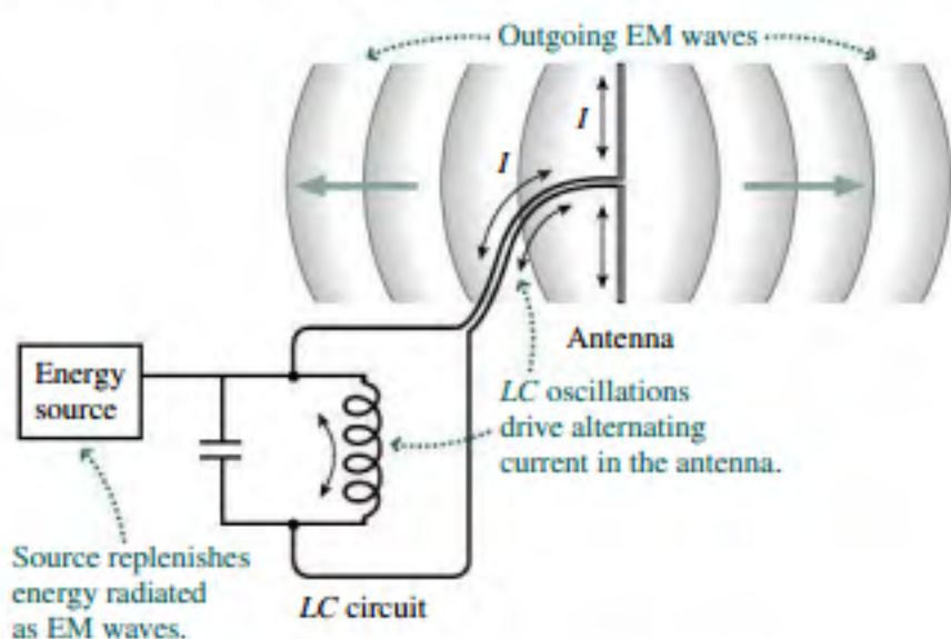
FIGURE 29.11 Simplified diagram of a radio transmitter.
