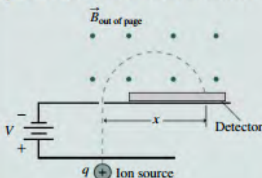
FIGURE 26.7 A mass spectrometer.
