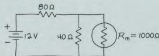
FIGURE 25.16 A nonideal voltmeter ( R_m ) alters the circuit.
