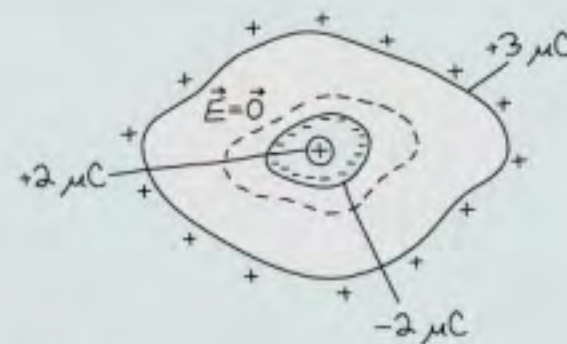
FIGURE 21.25 The Gaussian surface encloses zero net charge, so there must be -2\ \mu\text{C} on the cavity wall.
