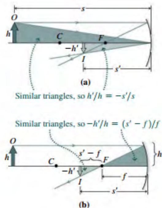
FIGURE 31.10 Finding the image I using rays 1 and 3 of Tactics 31.1. For an inverted image the height h' is negative, so we've marked the image arrow's length—a positive quantity—as -h' .
