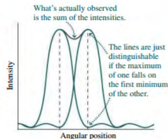
FIGURE 32.10 Intensity versus angular position for spectral lines with slightly different wavelengths, as dispersed with a grating.
