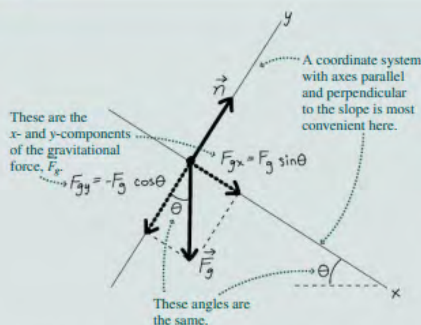
FIGURE 5.2 Our free-body diagram for the skier.
