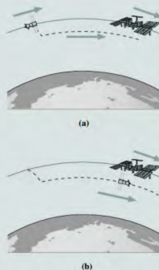
FIGURE 8.14 Playing catch-up with the space station.
