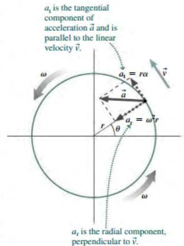
FIGURE 10.4 Radial and tangential acceleration.
