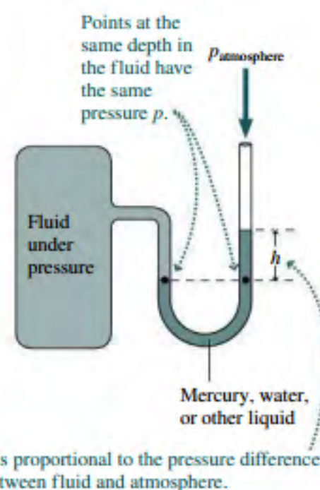
FIGURE 15.5 A manometer used to measure the pressure difference between a closed container and the atmosphere.
