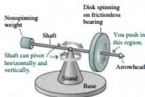
FIGURE 11.21 A gyroscope (Passage Problems 65–68)
