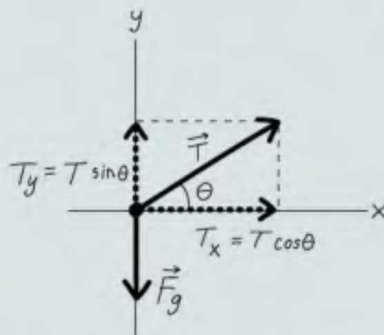
FIGURE 5.12 Our free-body diagram for the whirling ball.
