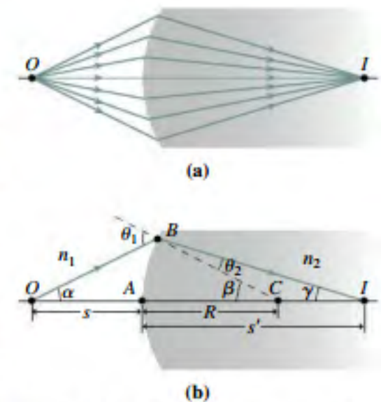
FIGURE 31.22 Refraction at an interface with a curved surface. All labeled angles are considered small, even though the drawing doesn't show them as such.
