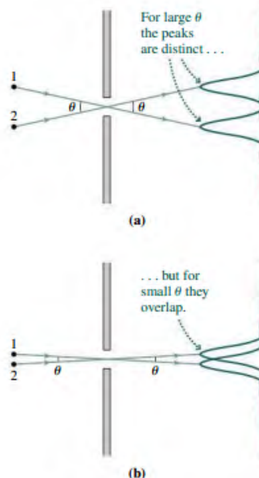
FIGURE 32.24 Two distant light sources at different angular positions produce diffraction patterns whose central peaks have the same angular separation \theta as the sources.
