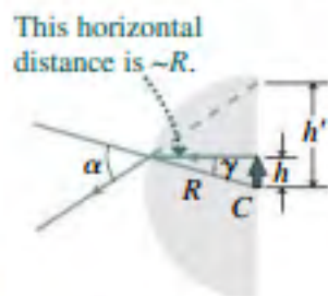
FIGURE 31.36 The figure shows one ray emerging horizontally from the arrowhead and refracting at the surface of the magnifier. Also shown is the normal to the glass-air interface, drawn from the center ( C ) and extending radially outward.
