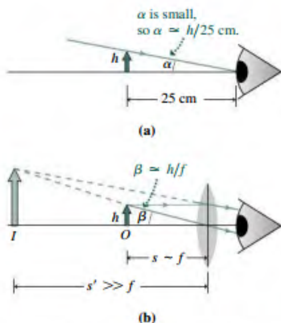
FIGURE 31.30 Calculating the angular magnification m = \beta/\alpha .
