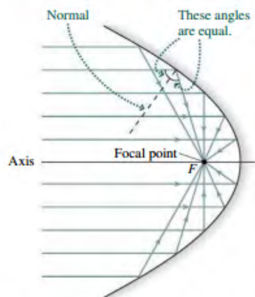
FIGURE 31.3 A parabolic mirror reflects rays parallel to its axis to a common focus.
