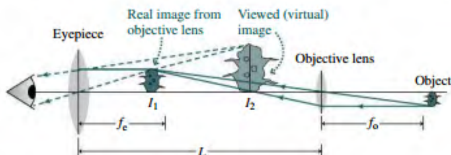
FIGURE 31.31 Image formation in a compound microscope. Figure is not to scale: L should be much greater than either focal length.
