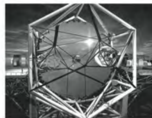
FIGURE 31.33 Artist's conception of the Thirty Meter Telescope, whose mirror consists of 492 individual segments. The TMT should be operational in the mid-2020s.
