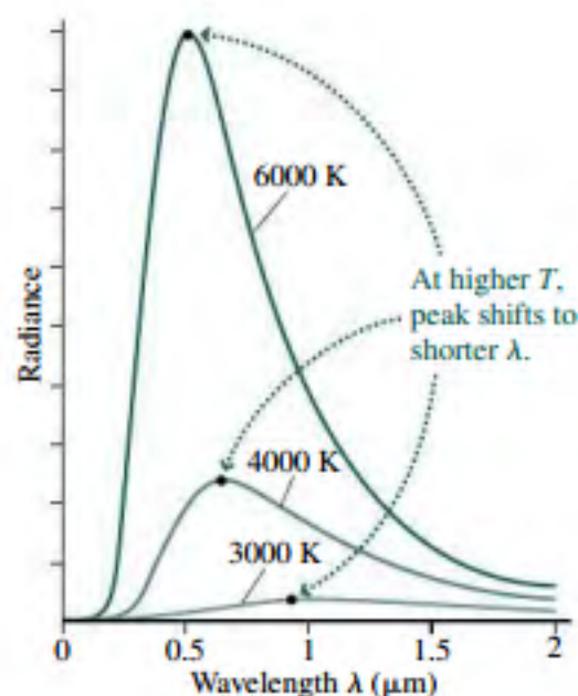
FIGURE 34.2 Blackbody radiance—power per unit area per unit wavelength interval—as a function of wavelength.
