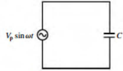
FIGURE 28.3 A capacitor connected across an AC generator.
