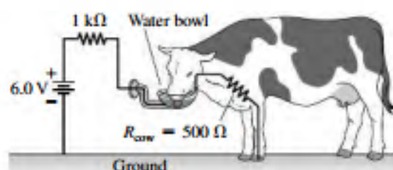
FIGURE 25.41 Stray voltage can bankrupt a dairy farm (Passage Problems 84–87)
