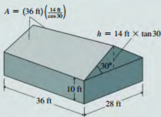
FIGURE 16.9 House for Example 16.4.
