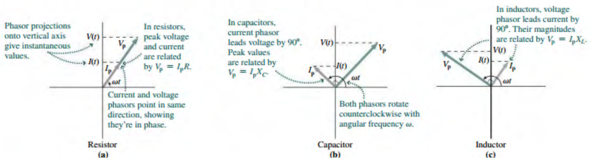
FIGURE 28.7 Phasor diagrams showing voltage and current in (a) a resistor, (b) a capacitor, and (c) an inductor. In all three diagrams both phasors rotate counterclockwise with angular frequency \omega .
