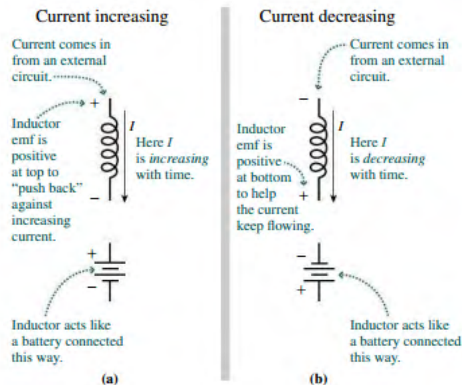
FIGURE 27.20 The direction of the induced emf in an inductor depends on whether the current is (a) increasing or (b) decreasing.
