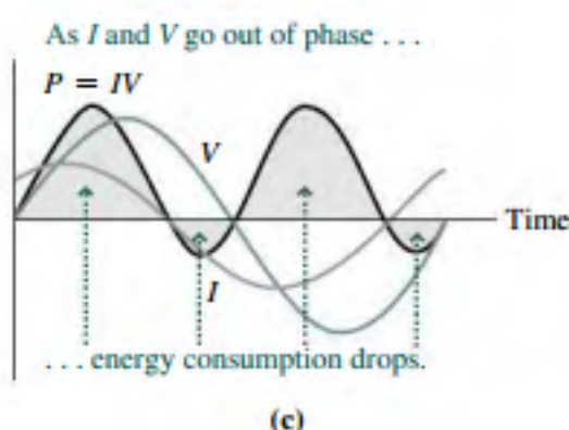
FIGURE 28.19 Energy consumption over one cycle is the area under the curve P = IV , with areas below the axis counted as negative.
