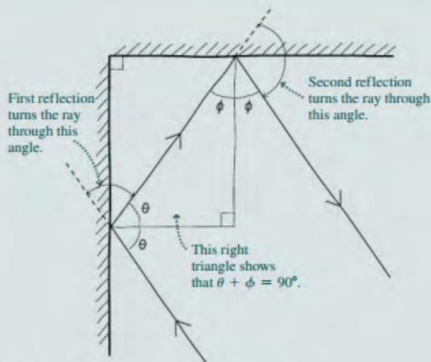
FIGURE 30.2 A two-dimensional corner reflector.
