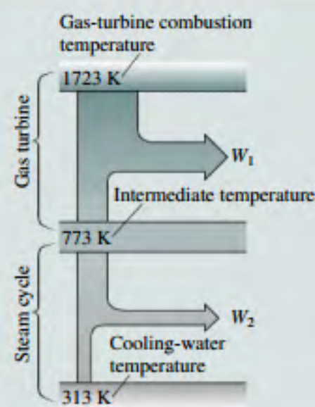
FIGURE 19.11 Conceptual diagram of a combined-cycle power plant.
