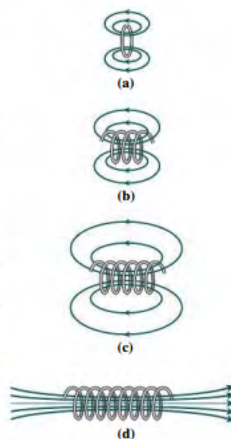
FIGURE 26.34 As the coil gets longer, the interior field stays nearly constant but the exterior field weakens as the field lines spread ever farther apart.
