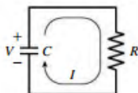
FIGURE 25.22 A discharging RC circuit.
