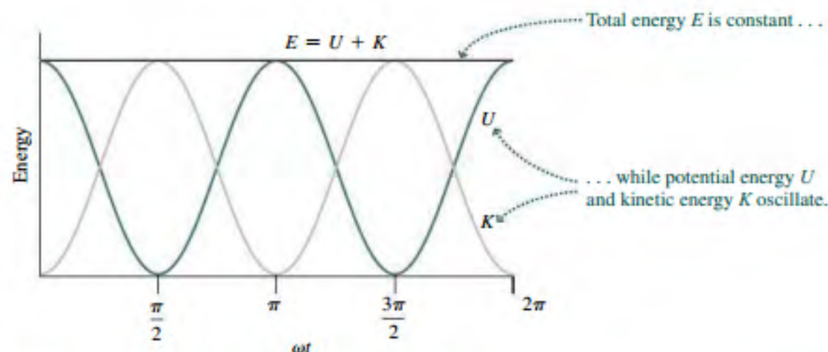
FIGURE 13.20 Energy of a simple harmonic oscillator.
