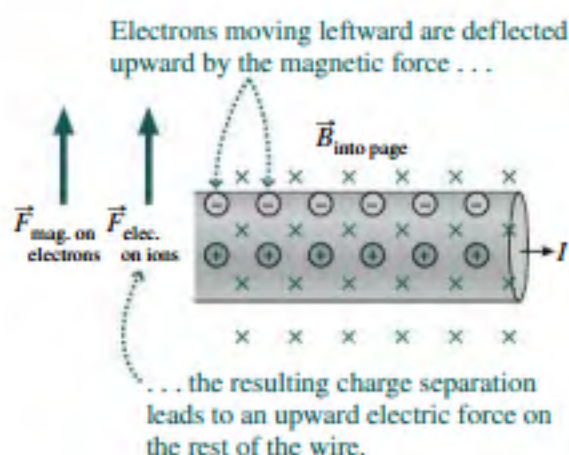
FIGURE 26.12 Origin of the magnetic force on a current-carrying wire.
