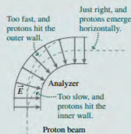
FIGURE 20.20 An electrostatic analyzer.
