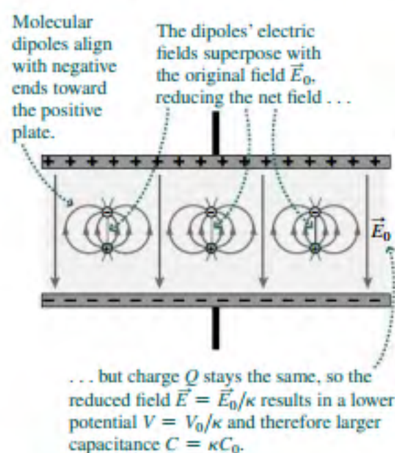
FIGURE 23.6 A capacitor with a dielectric.
