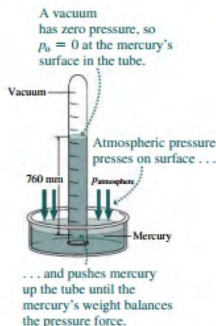
FIGURE 15.4 A mercury barometer.
