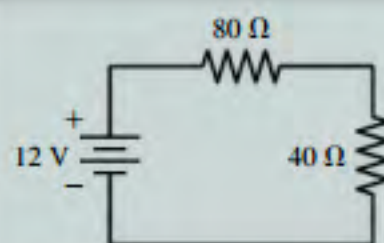
FIGURE 25.15 What's the voltage across the 40- \Omega resistor?
