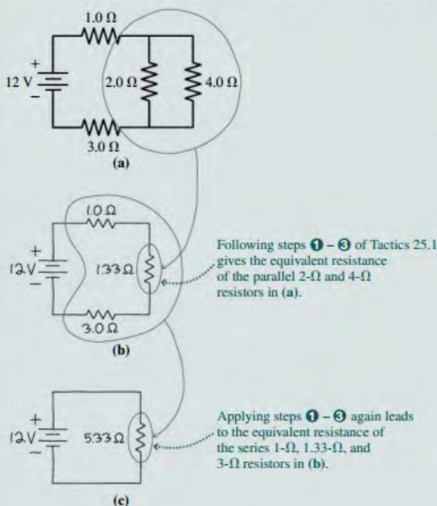
FIGURE 25.11 Analyzing a circuit.
