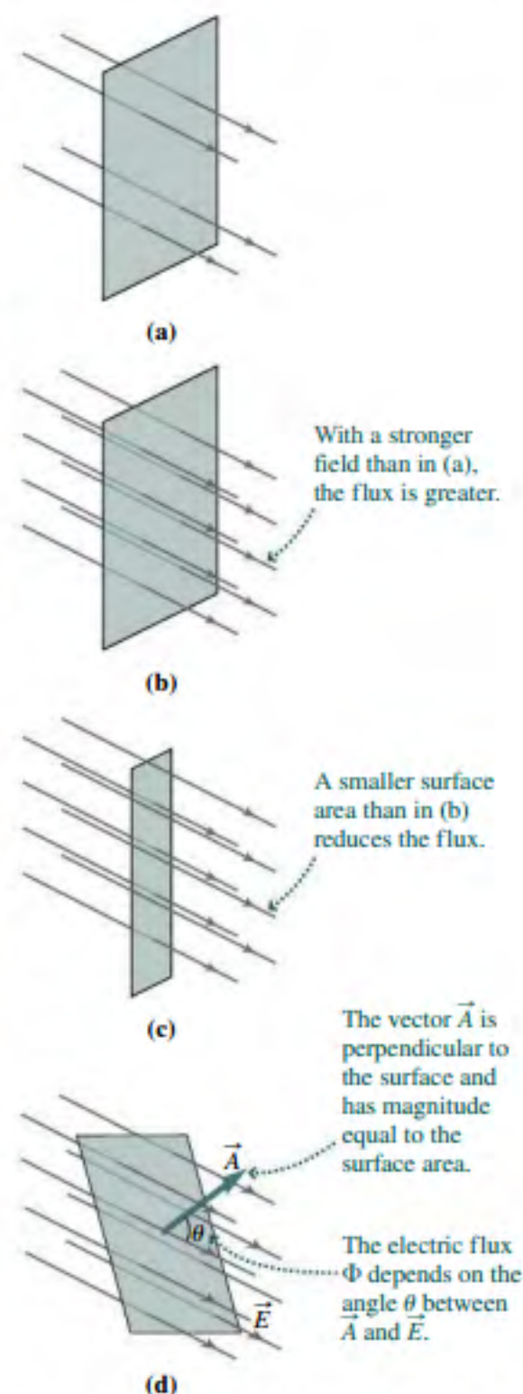
FIGURE 21.5 Electric flux through flat surfaces.
