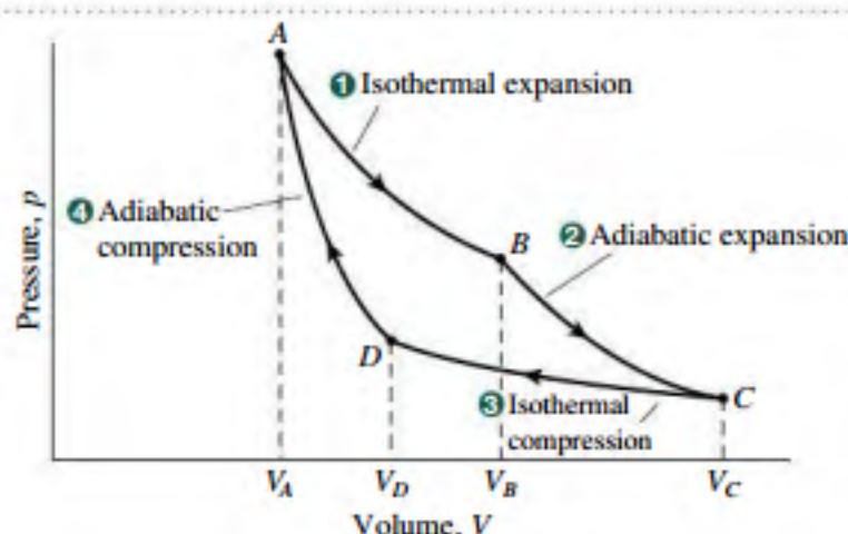
pV diagram for Carnot engine
