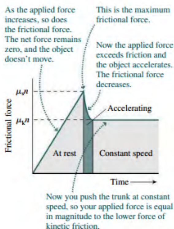
FIGURE 5.19 Behavior of frictional forces.
