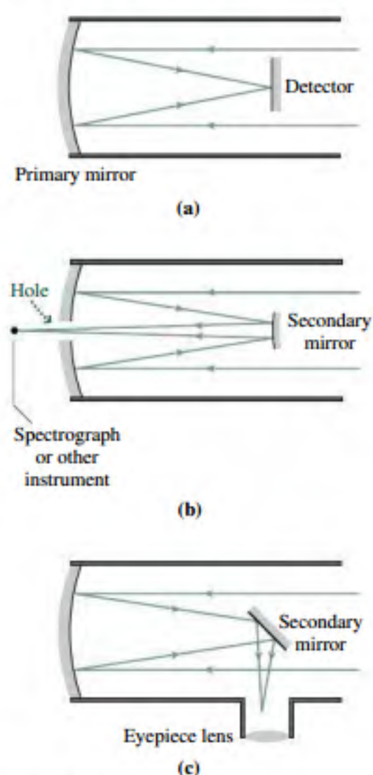
FIGURE 31.34 Reflecting telescopes.
