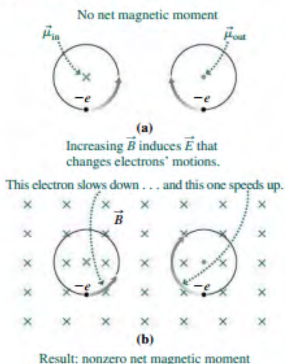
FIGURE 27.32 A simple model for diamagnetism.
