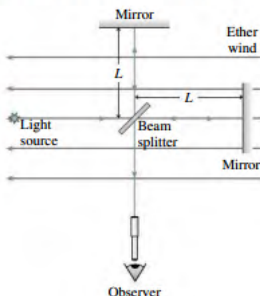
FIGURE 33.2 Simplified diagram of the Michelson–Morley experiment. Ether wind should result in a longer travel time for light on the horizontal arm.
