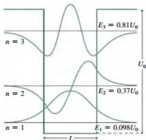
FIGURE 35.14 Bound-state wave functions for a finite square well, superposed on the associated energy levels. For this combination of well depth, well width, and particle mass, there are only three bound states.
