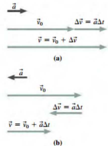
FIGURE 3.7 When \vec{v} and \vec{a} are collinear, generally only the speed changes. (However, if the acceleration acts long enough, the object may come to a stop and then reverse direction.)
