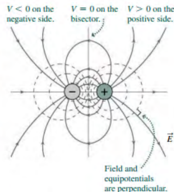
FIGURE 22.16 Equipotentials (dashed curves) and field lines for a dipole, in a plane containing the dipole. You should convince yourself that the equipotentials provide a contour map of Fig. 22.11.
