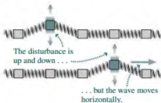
FIGURE 14.2 A transverse wave.
