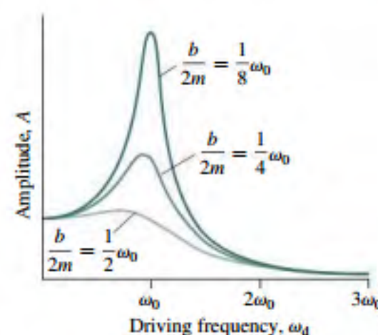
FIGURE 13.25 Resonance curves for three damping strengths; \omega_0 is the undamped natural frequency \sqrt{k/m} .
