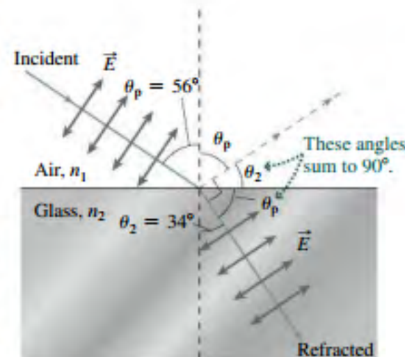
FIGURE 30.8 The polarizing incidence angle \theta_p occurs when the angles of incidence and refraction sum to 90^\circ .
