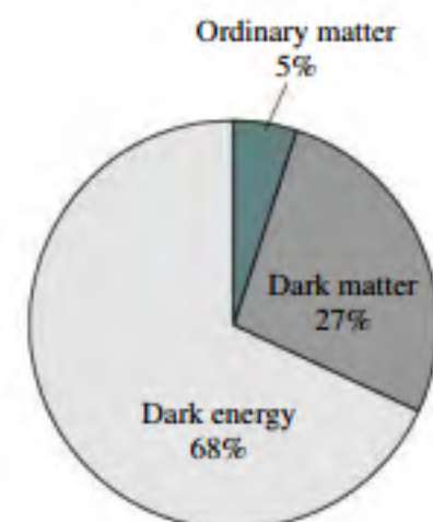
FIGURE 39.17 Composition of the universe, from the Planck spacecraft supplemented with additional data. Only a tiny fraction (colored wedge) is “stuff” we understand!
