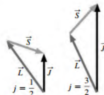
FIGURE 36.10 Spin-orbit coupling with l = 1 , for which Equation 36.17a gives j = \frac{1}{2} or j = \frac{3}{2} .
