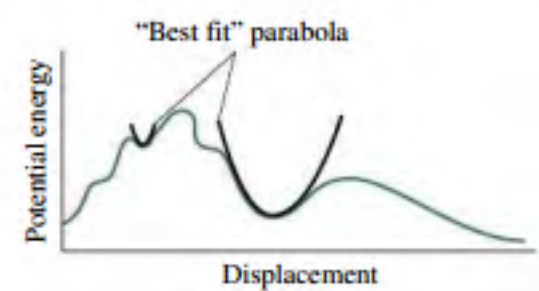
FIGURE 13.21 Near their minima, potential-energy curves often approximate parabolas. This results in simple harmonic motion.
