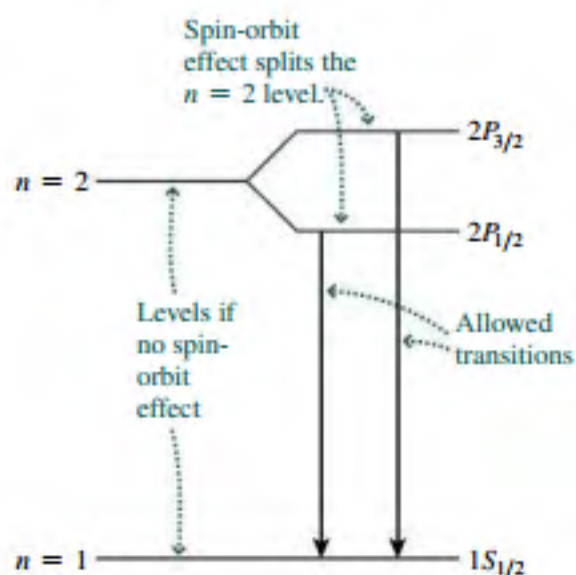
FIGURE 36.12 Energy-level diagram showing spin-orbit splitting of the 2P levels in hydrogen. Diagram is not to scale; the spacing between the 2P_{1/2} and 2P_{3/2} levels is actually about five millionths that of the n = 1 and n = 2 levels.
