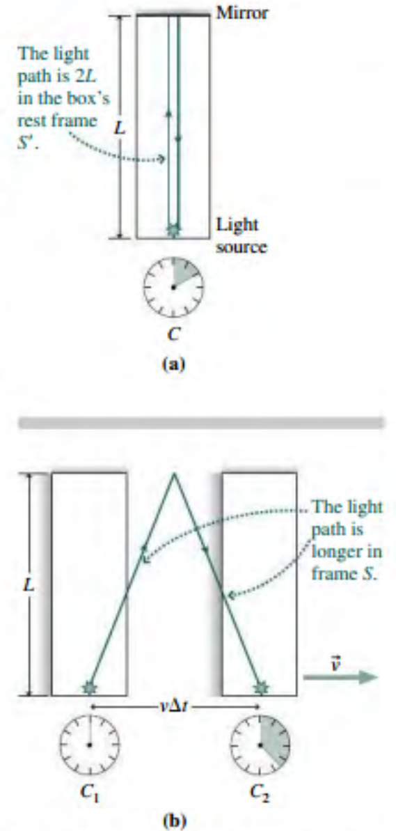
FIGURE 33.6 A “light box” to explore time dilation shown (a) in a reference frame S' at rest with respect to the box and (b) in a frame S where the box is moving to the right.
