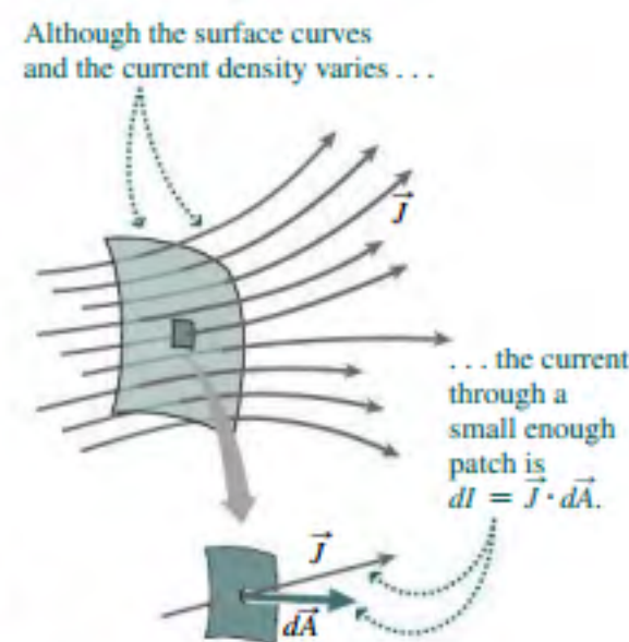
FIGURE 24.4 Current I is the flux of the current density \vec{J} , and finding the total current in the case of nonuniform \vec{J} requires integration. Compare with Fig. 21.6.
