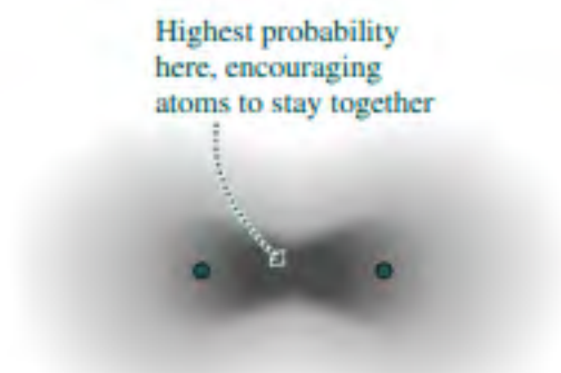
FIGURE 37.4 Probability density for finding electrons in the ground state of molecular hydrogen ( \text{H}_2 ).
