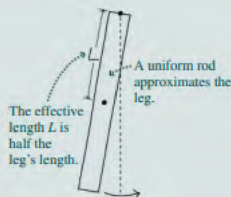
FIGURE 13.15 A human leg treated as a pendulum.
