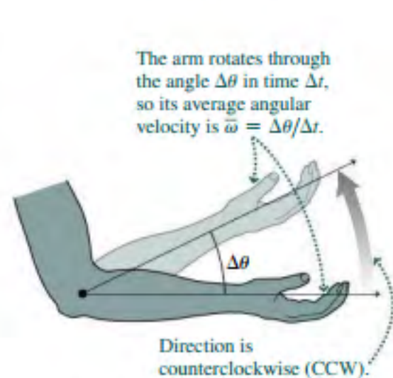
FIGURE 10.2 Average angular velocity.
