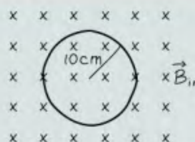
FIGURE 27.8 A circular conducting loop in a plane perpendicular to a uniform magnetic field.
