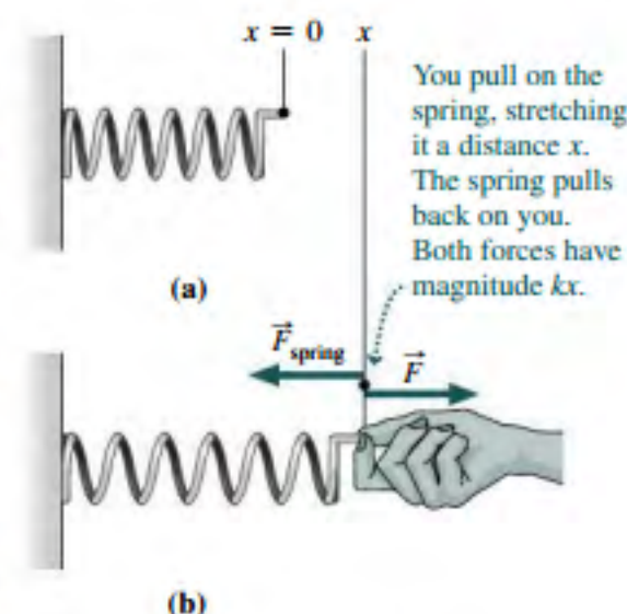
FIGURE 6.10 Stretching a spring.
