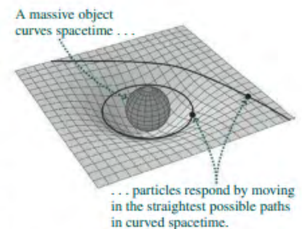
FIGURE 33.22 A two-dimensional analog of curved spacetime in general relativity.
