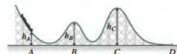
FIGURE 7.9 A roller-coaster track.
