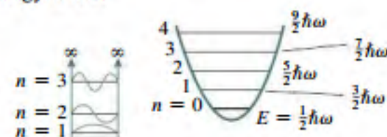
Infinite square well Harmonic oscillator
