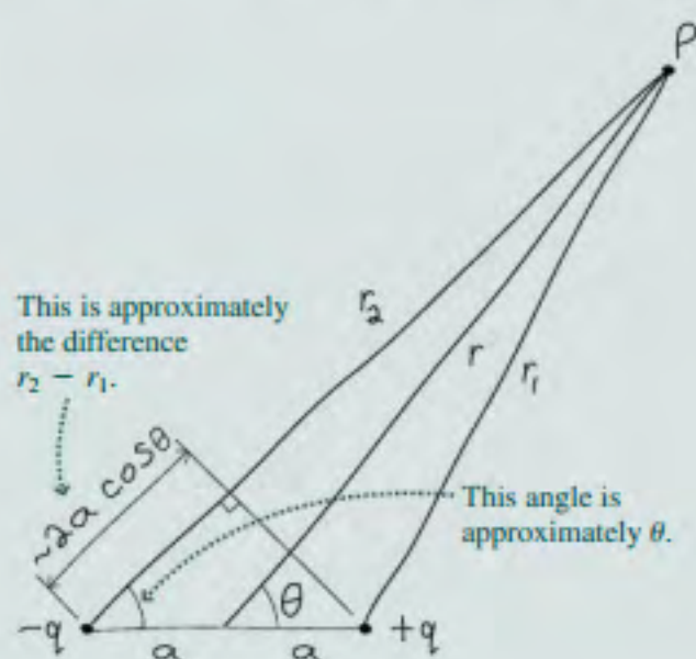
FIGURE 22.10 Finding the dipole potential.
