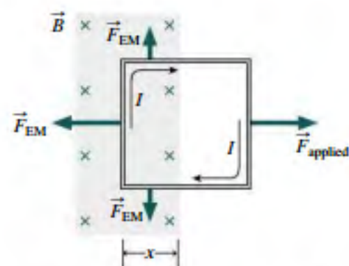
FIGURE 27.13 Forces on the loop. The subscript EM indicates that the forces on the conducting loop result from both electric and magnetic fields.
