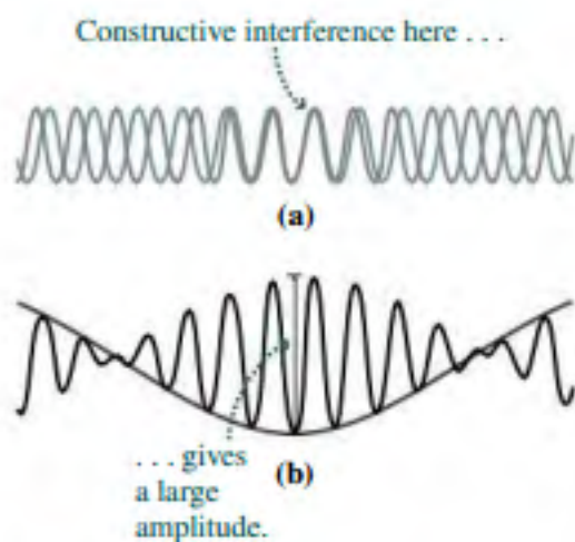
FIGURE 14.20 The origin of beats.
