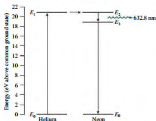
FIGURE 36.19 Energy-level diagram for the helium–neon laser (Problem 74).
