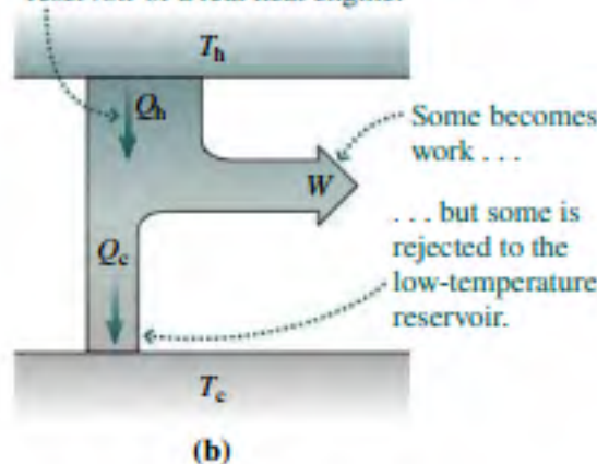
FIGURE 19.3 (a) Energy-flow diagram for a perfect heat engine. (b) A real engine delivers as work only a fraction of the energy extracted from the high-temperature reservoir.
