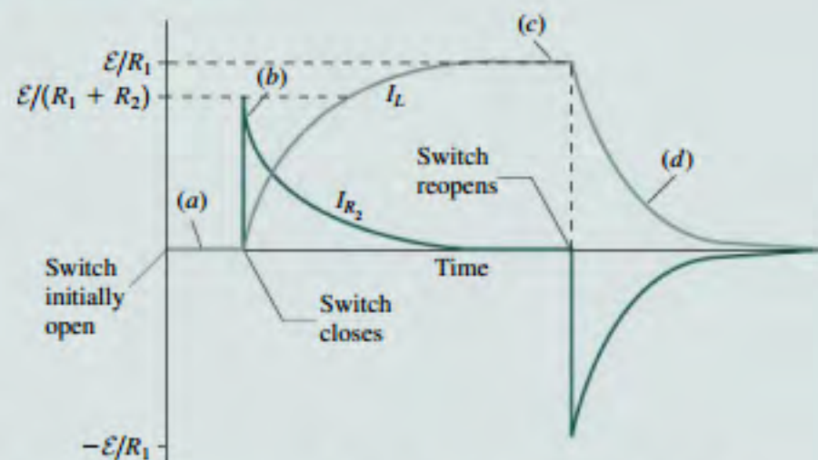
FIGURE 27.28 Currents in R_2 and L for Conceptual Example 27.1.
