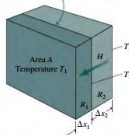
FIGURE 16.7 A composite slab.
