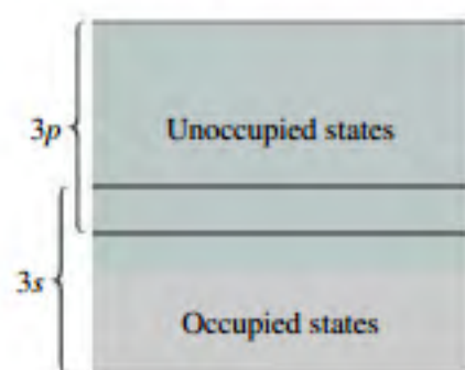
FIGURE 37.15 Band structure of metallic sodium, with gray indicating filled states and color unfilled states. Bands lower than 3s aren't shown; they correspond to inner electrons, whose levels aren't split significantly.
