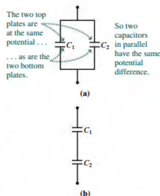
FIGURE 23.7 Connecting capacitors: (a) parallel and (b) series. \frac{1}{\square} is the standard circuit symbol for a capacitor.
