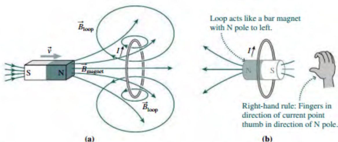
FIGURE 27.10 Conservation of energy determines the direction of the induced current. (a) Fields of a bar magnet and a conducting loop, shown when the magnet is moving toward the loop. (b) The loop acts like a magnet with north pole to the left, making it hard to move the bar magnet.
