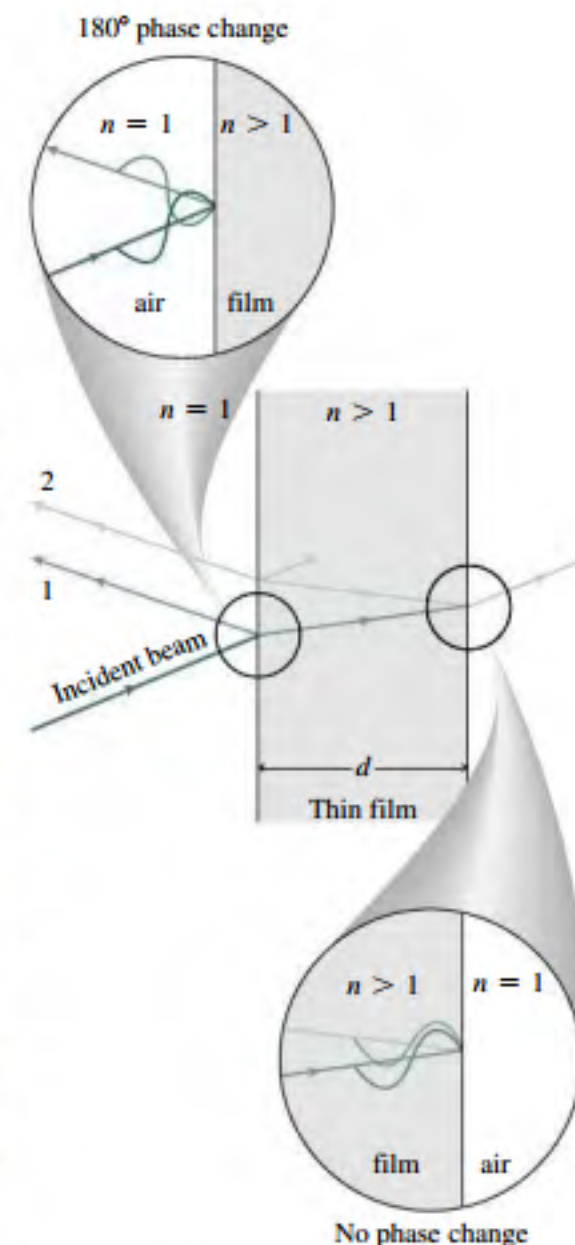
FIGURE 32.12 Reflection and refraction at a thin film of transparent material, showing a 180^\circ phase change at the first interface and none at the second.
