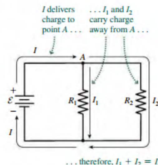
FIGURE 25.10 Parallel resistors connected across a battery.
