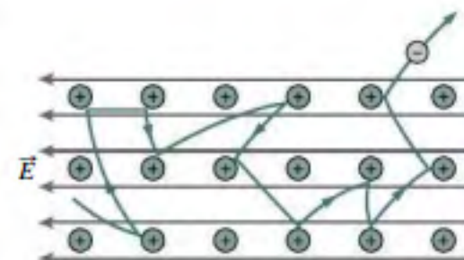
FIGURE 24.7 An electron's path in a metal is almost completely random, but in the presence of an electric field there's a slight drift antiparallel to the field. The electrons actually collide not with ions themselves but with phonons associated with vibrations of the ion lattice.
