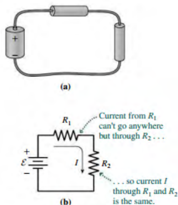
FIGURE 25.4 A battery and two resistors in series: (a) physical circuit; (b) schematic diagram.
