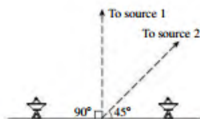
FIGURE 32.29 A two-dish interferometer used for radio astronomy (Passage Problems 73–76). Dashed lines show directions to sources in Problems 75 and 76.
