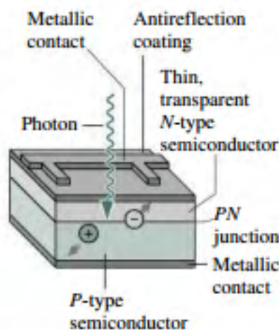
FIGURE 37.26 Operation of a photovoltaic cell, showing a solar photon producing an electron-hole pair at the PN junction (Passage Problems 67–70).
