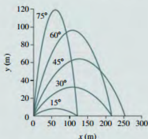
FIGURE 3.20 Trajectories for a projectile launched at 50 m/s.
