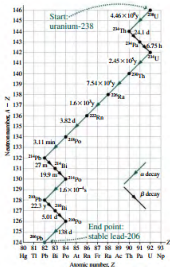
FIGURE 38.7 The decay of uranium-238 results in a chain of shorter-lived nuclei. Times shown are half-lives.
