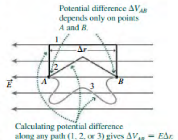
FIGURE 22.2 Potential difference is path independent.
