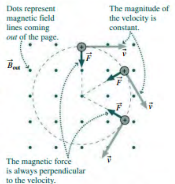
FIGURE 26.6 A charged particle moving at right angles to a uniform magnetic field describes circular motion.
