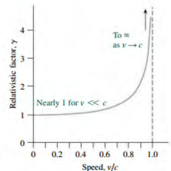
FIGURE 33.15 The relativistic factor \gamma differs significantly from 1 only as relative speeds approach c .
