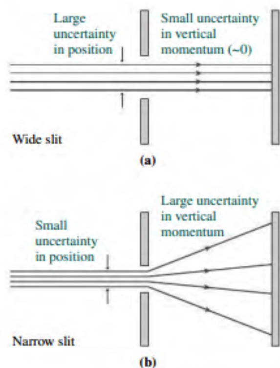
FIGURE 34.14 The wave nature of matter is intimately related to the uncertainty principle, as shown here for beams of electrons passing through wide and narrow slits. In (b), diffraction introduces the uncertainty in vertical momentum.
