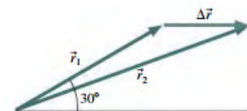
FIGURE 3.2 Vectors \vec{r}_1 and \Delta\vec{r} sum to \vec{r}_2 .
