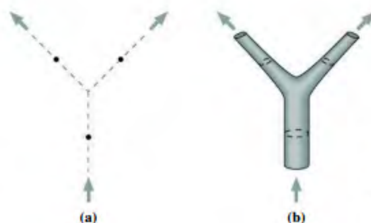
FIGURE 39.9 (a) A particle decay involving point particles in the standard model. (b) A similar decay in string theory. Note that there's no single point in spacetime at which the decay takes place.
