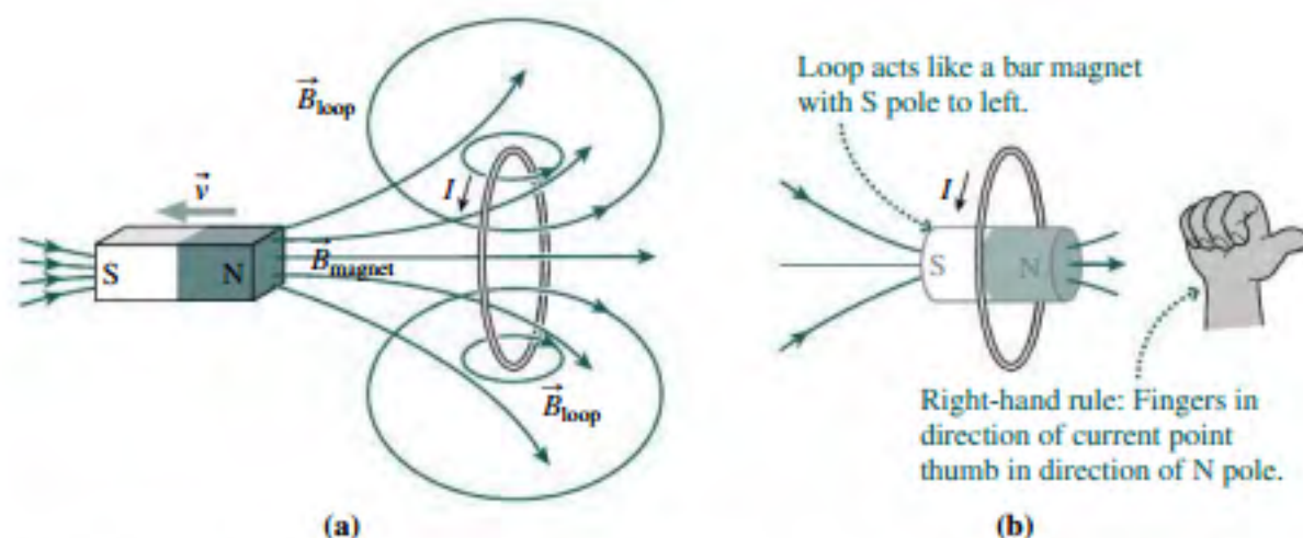
FIGURE 27.11 When the bar magnet is moving away from the loop, the direction of the induced current puts the loop's south pole to the left, making it hard to pull the magnet away.
