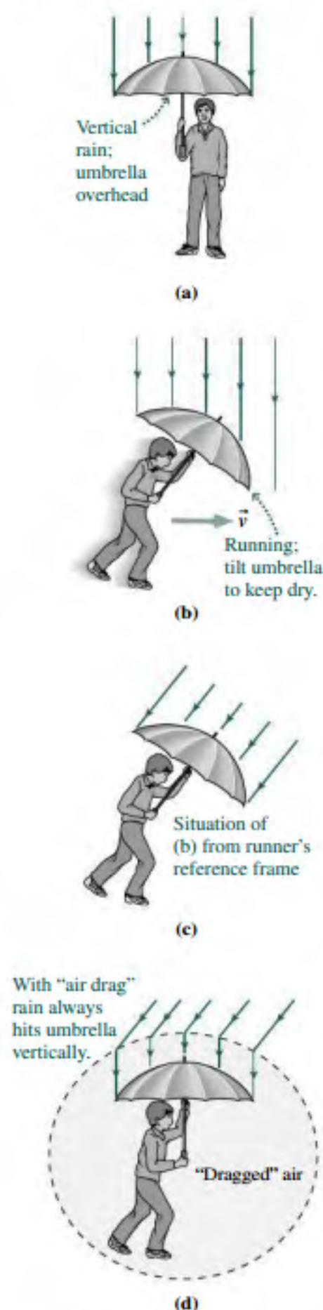
FIGURE 33.1 A rain/umbrella analogy for aberration of starlight.
