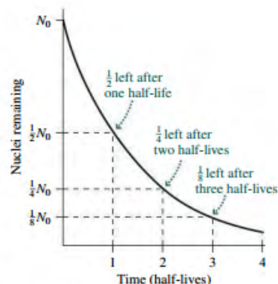
FIGURE 38.5 Exponential decay of a radioactive sample.
