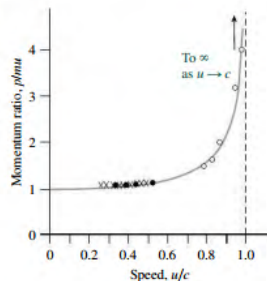
FIGURE 33.19 The ratio of relativistic momentum to Newtonian momentum mu . The curve follows Equation 33.7; crosses and circles mark experimental data. Compare with Figure 33.15.
