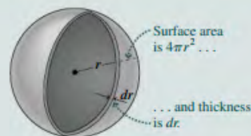
FIGURE 23.11 A thin spherical shell has volume dV = 4\pi r^2 dr .
