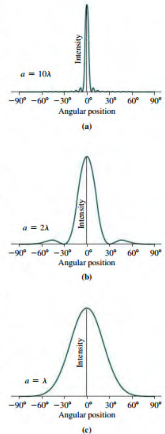
FIGURE 32.21 Intensity in single-slit diffraction, as a function of the angle \theta from the centerline, for three values of slit width a .
