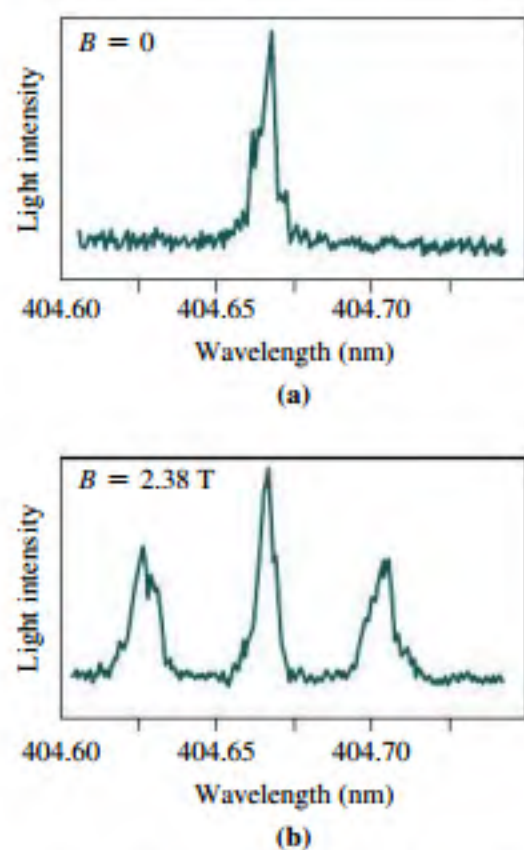
FIGURE 35.18 (a) Spectral line at 404.66 nm produced by mercury atoms undergoing transitions from n = 7 to n = 6 . The upper level is actually threefold degenerate. (b) A magnetic field breaks the symmetry and removes the degeneracy, splitting the spectral line.
