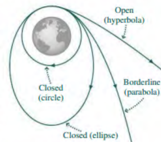
FIGURE 8.8 Closed and open orbits.
