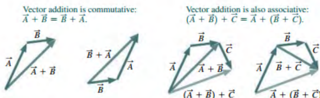
FIGURE 3.3 Vector addition is commutative and associative.
