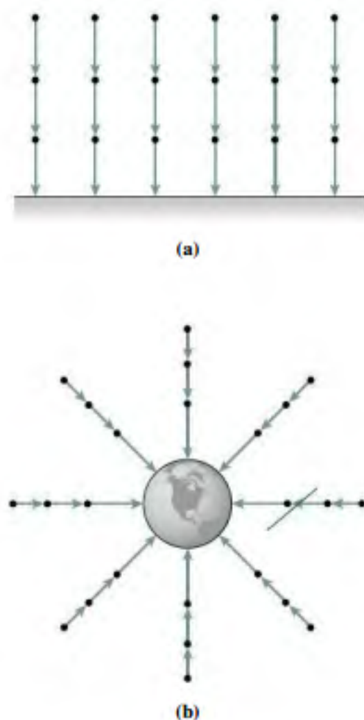
FIGURE 8.15 Gravitational field vectors at points (a) near Earth's surface and (b) on a larger scale.
