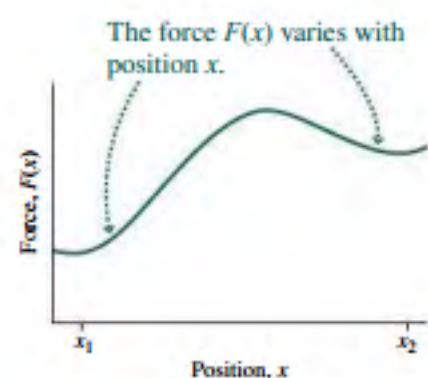
FIGURE 6.8 A varying force.
