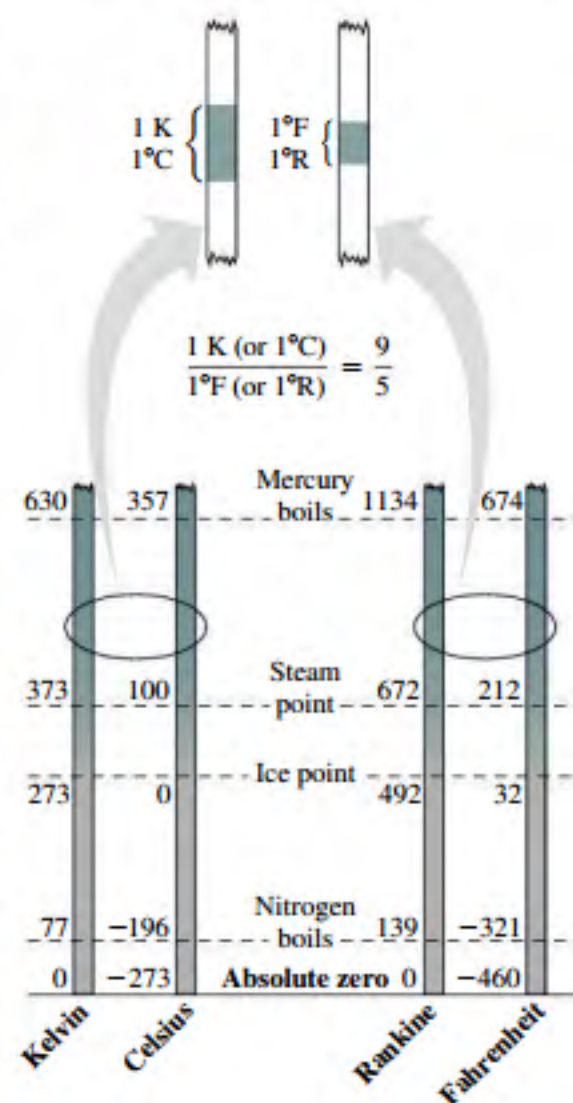
FIGURE 16.4 Relationships among four temperature scales.
