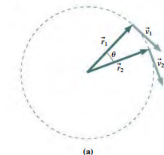
FIGURE 3.21 Velocity vectors in circular motion are tangent to the circular path.
