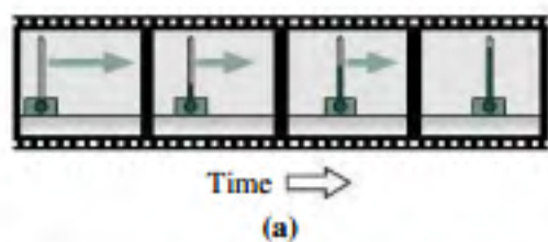
FIGURE 19.1 A movie of a bouncing ball makes sense whether it's shown (a) forward or (b) backward.
