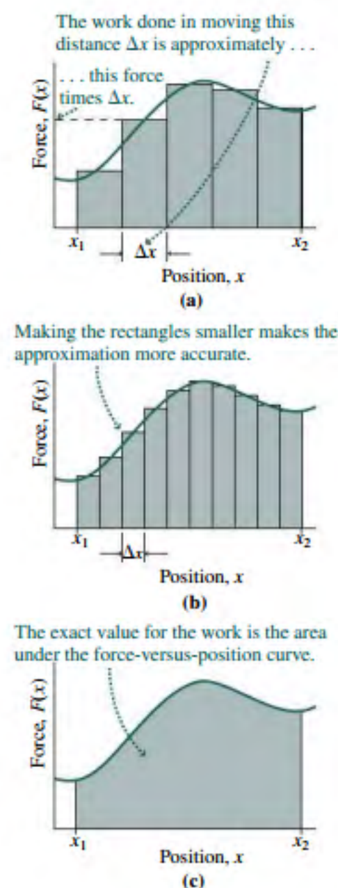
FIGURE 6.9 Work done by a varying force.
