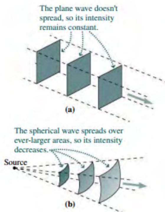
FIGURE 14.13 (a) Plane and (b) spherical waves.
