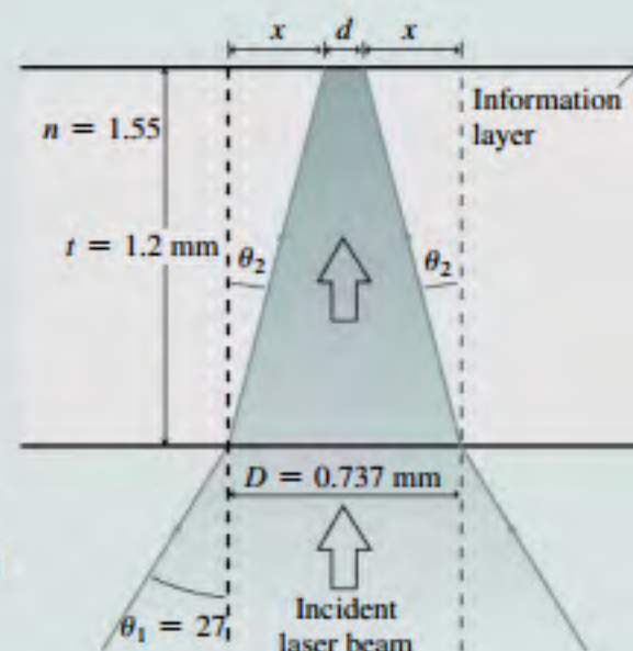
FIGURE 30.7 Section through a compact disc, showing convergence of the laser beam to a narrow spot at the information layer.
