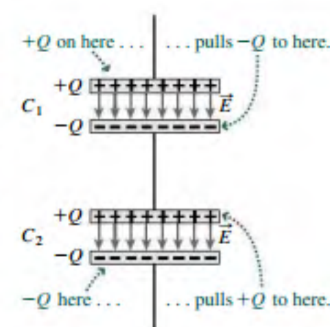
FIGURE 23.8 Capacitors in series carry the same charge.
