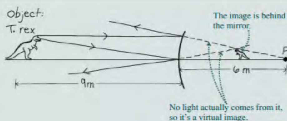
FIGURE 31.13 Sketch for Example 31.2, showing two rays that locate the image of T. rex . Mirror is not to scale.
