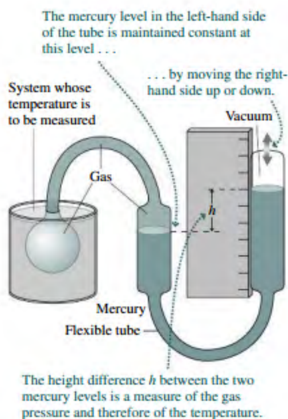
FIGURE 16.2 A constant-volume gas thermometer.
