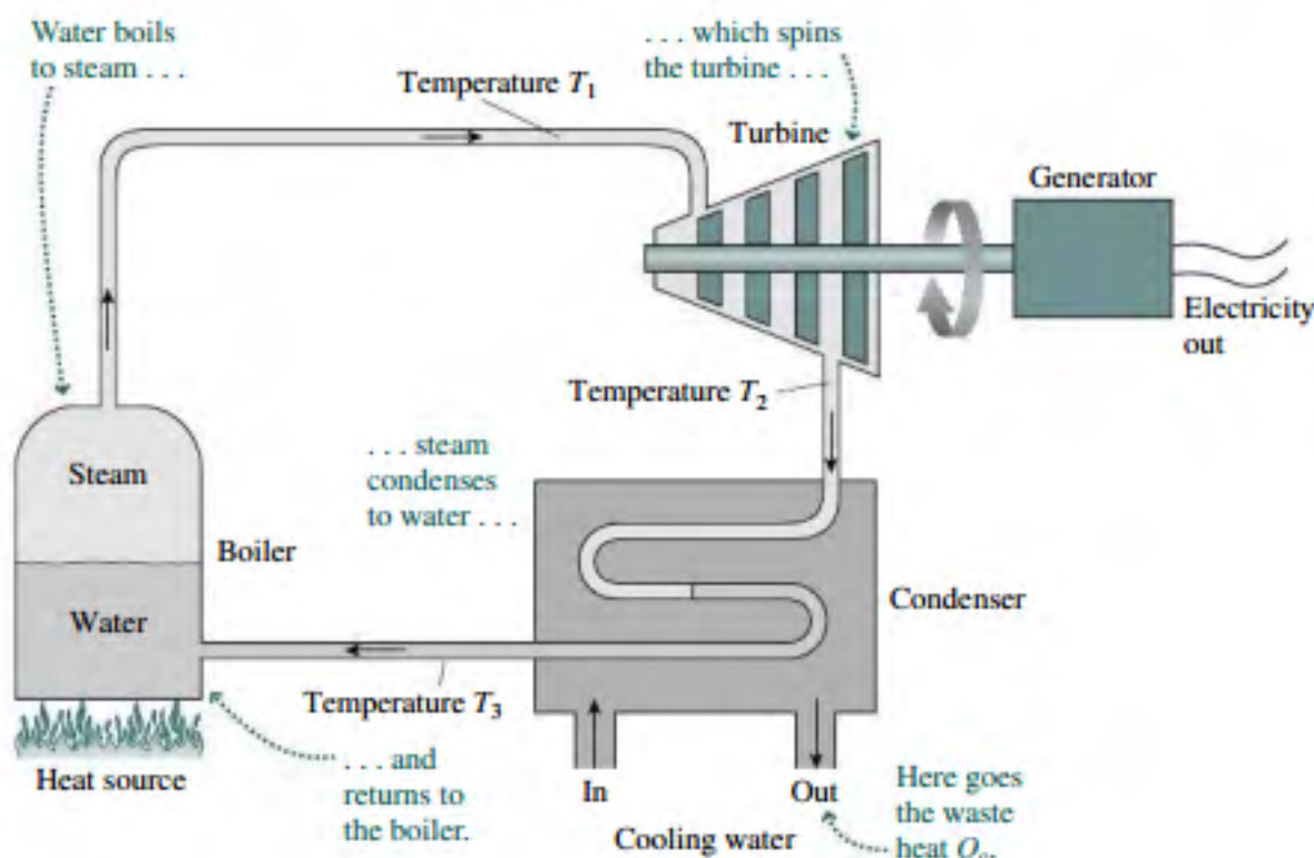
FIGURE 19.10 Schematic diagram of an electric power plant.
