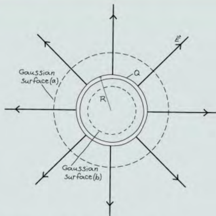
FIGURE 21.11 Finding the field of a charged shell.
