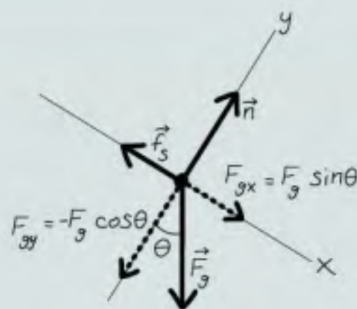
FIGURE 5.26 Our free-body diagram for the snow slab.
