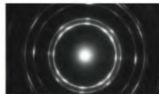
FIGURE 34.12 Diffraction produced by passing an electron beam through a circular aperture shows that electrons have a wave-like character.
