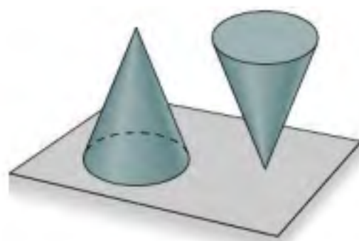
FIGURE 12.6 Stable (left) and unstable (right) equilibria.
