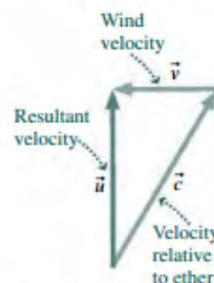
FIGURE 33.3 Vector diagram for light moving at right angles to an ether wind.
