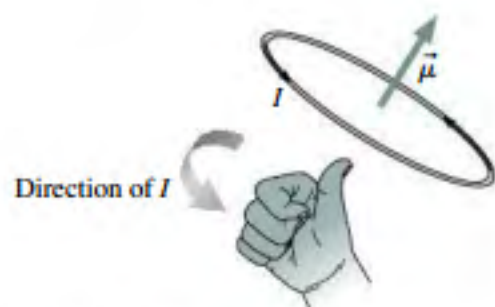
FIGURE 26.21 Finding the direction of a current loop's magnetic dipole moment.
