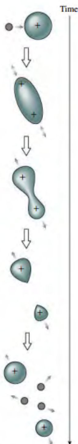
FIGURE 38.11 Neutron-induced fission of ^{235}\text{U} , showing three neutrons (gray) released in the process.
