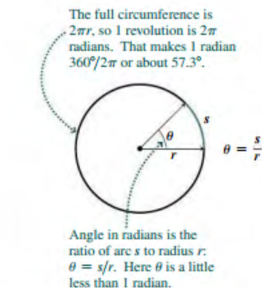
FIGURE 10.1 Radian measure of angles.
