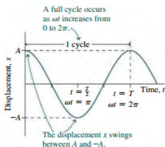
FIGURE 13.5 The function A \cos \omega t .
