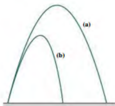
FIGURE 5.29 Projectile trajectories (a) without air resistance and (b) with substantial air resistance. Note that (b) not only achieves less height and range but that the trajectory is no longer a symmetric parabola.
