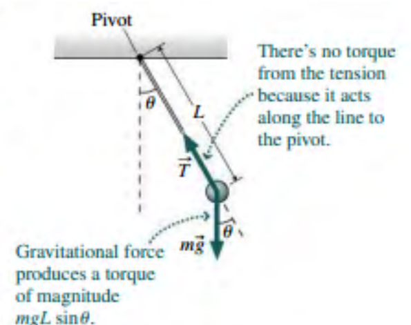
FIGURE 13.10 Forces on a pendulum.
