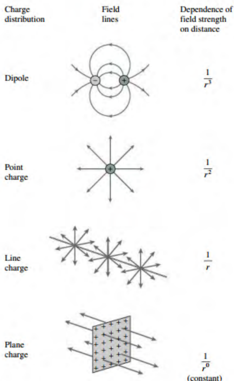
FIGURE 21.21 Electric fields of a dipole, a point charge, a charged line, and a charged plane.
