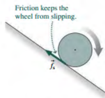
FIGURE 10.24 Rolling down a slope.
