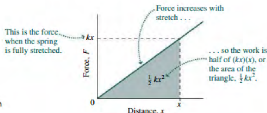
FIGURE 6.11 Work done in stretching a spring.
