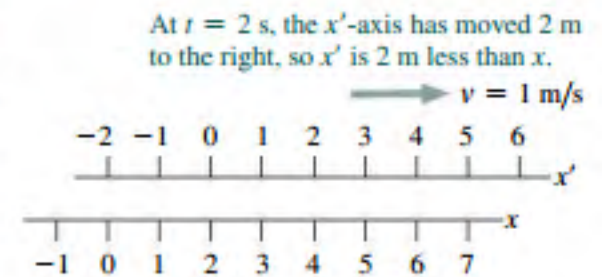
FIGURE 33.14 Nonrelativistic picture of two coordinate axes in relative motion, shown at time t = 2 s. In general, x' = x - vt .
