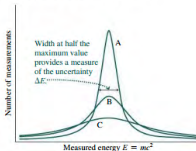
FIGURE 34.15 Mass distributions for high-energy particles (Passage Problems 82–85). The vertical axis gives the number of measurements that yield a given value on the horizontal axis.
