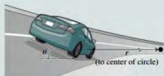
FIGURE 5.13 Car on a banked curve.
