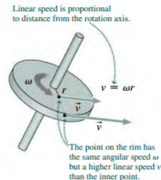
FIGURE 10.3 Linear and rotational speeds.
