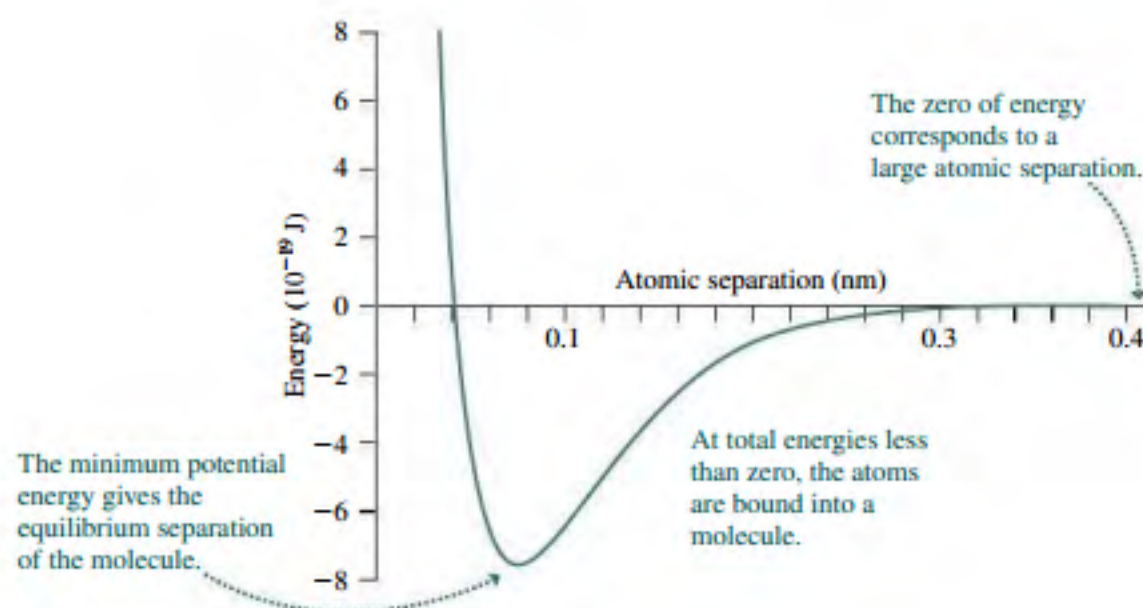
FIGURE 7.11 Potential-energy curve for two hydrogen atoms.
