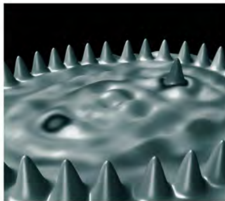
This scanning-tunneling microscope image shows a "quantum corral" of 36 cobalt atoms on a copper surface. What unusual quantum phenomenon enables this type of microscopy?
