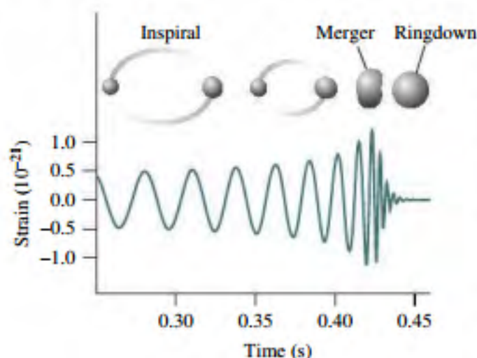
FIGURE 33.24 Signal from the first gravitational-wave detection, arising from the merger of two black holes the vertical axis measures strain—the fractional change in length of the detector arm as the gravitational wave passes. As indicated, the actual strain is 10^{-21} times the numbers shown on the vertical axis. The raw data have been smoothed for comparison with calculations based on general relativity. Drawings above the graph show the two black holes spiraling into an ever-closer orbit and finally merging.
