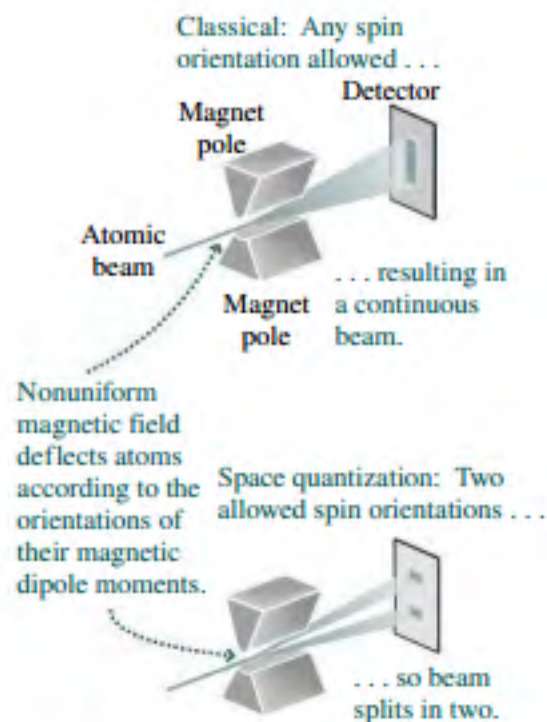
FIGURE 36.9 The Stern–Gerlach experiment.
