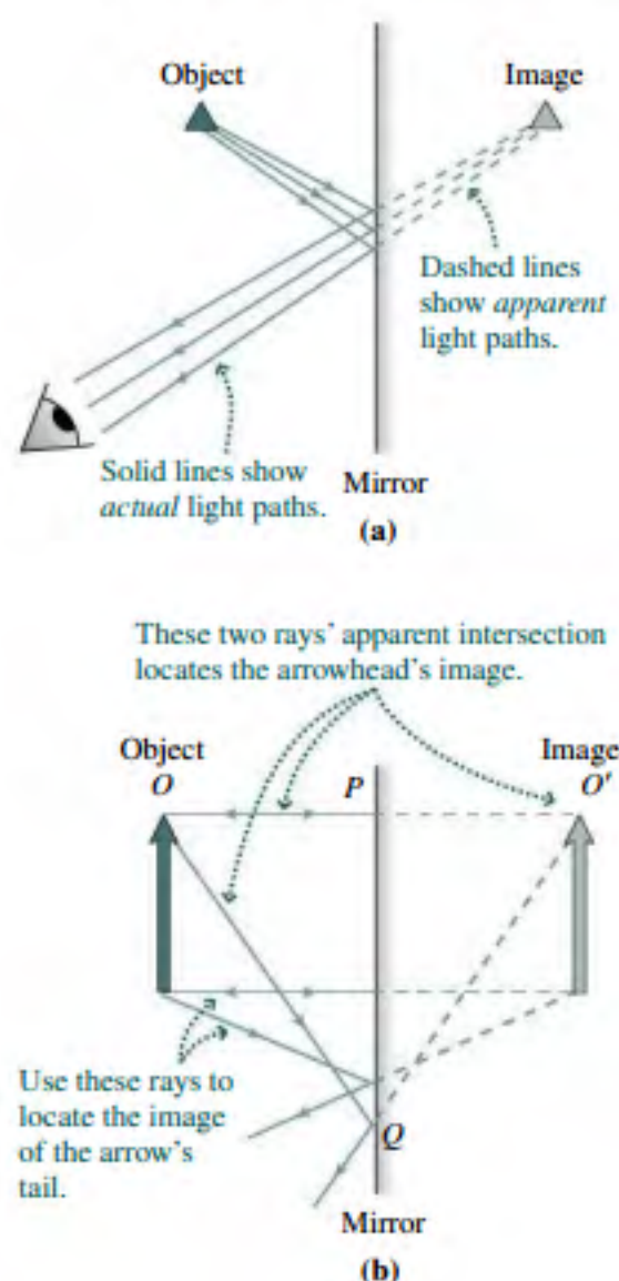
FIGURE 31.1 Image formation in a plane mirror.
