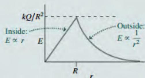
FIGURE 21.16 Field strength versus radial distance for a uniformly charged sphere of radius R .
