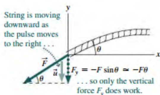
FIGURE 14.11 The vertical force component does work on the string; for small \theta , \sin \theta \approx \theta , so F_y \approx F\theta .
