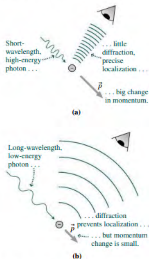
FIGURE 34.13 Heisenberg's "quantum microscope" thought experiment.
