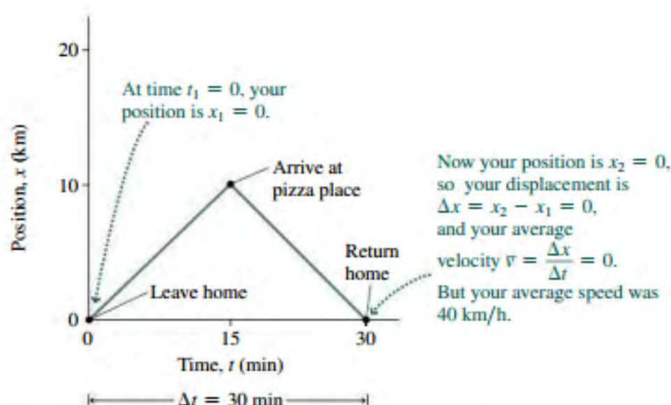
FIGURE 2.1 Position versus time for the pizza trip.
