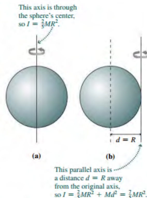
FIGURE 10.17 Meaning of the parallel-axis theorem.
