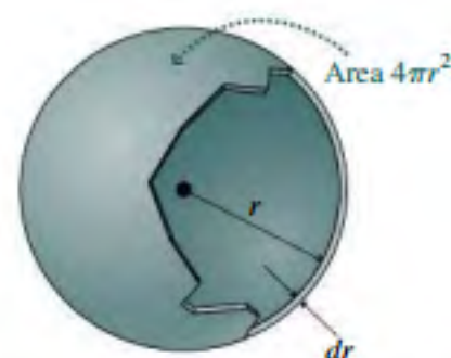
FIGURE 36.2 A thin shell has volume dV = 4\pi r^2 dr ; thus the probability per unit radial distance is 4\pi r^2 times the probability per unit volume.
