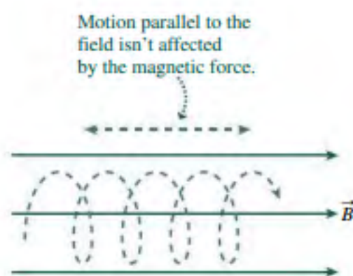
FIGURE 26.8 A charged particle in a uniform magnetic field describes a spiral path.
