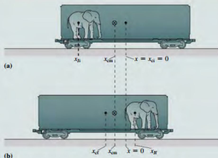
FIGURE 9.8 Jumbo walks, but the system's center of mass doesn't move.
