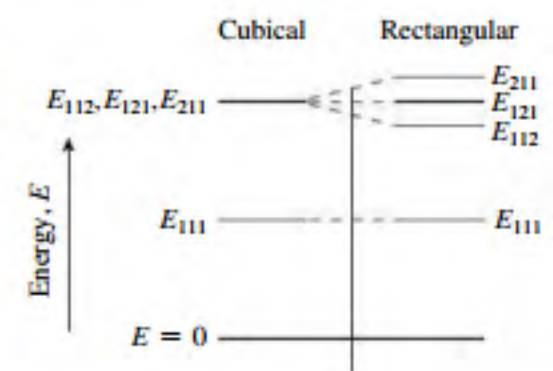
FIGURE 35.17 Energy-level diagrams showing the ground state and first excited state for a particle in a three-dimensional box. Making the sides different lengths removes the degeneracy.
