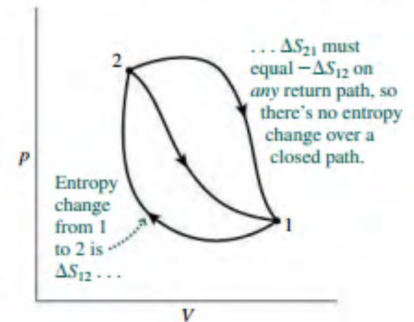
FIGURE 19.15 Entropy change is path-independent.
