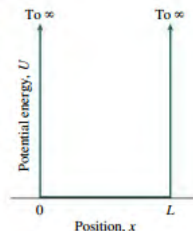
FIGURE 35.5 The infinite square-well potential-energy curve describes a particle constrained to move in one dimension between rigid walls separated by a distance L .
