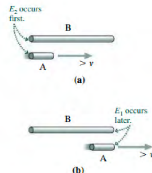
FIGURE 33.12 The passing rods viewed in a reference frame at rest with respect to rod B.
