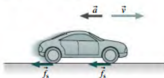
FIGURE 5.22 Friction stops the car.
