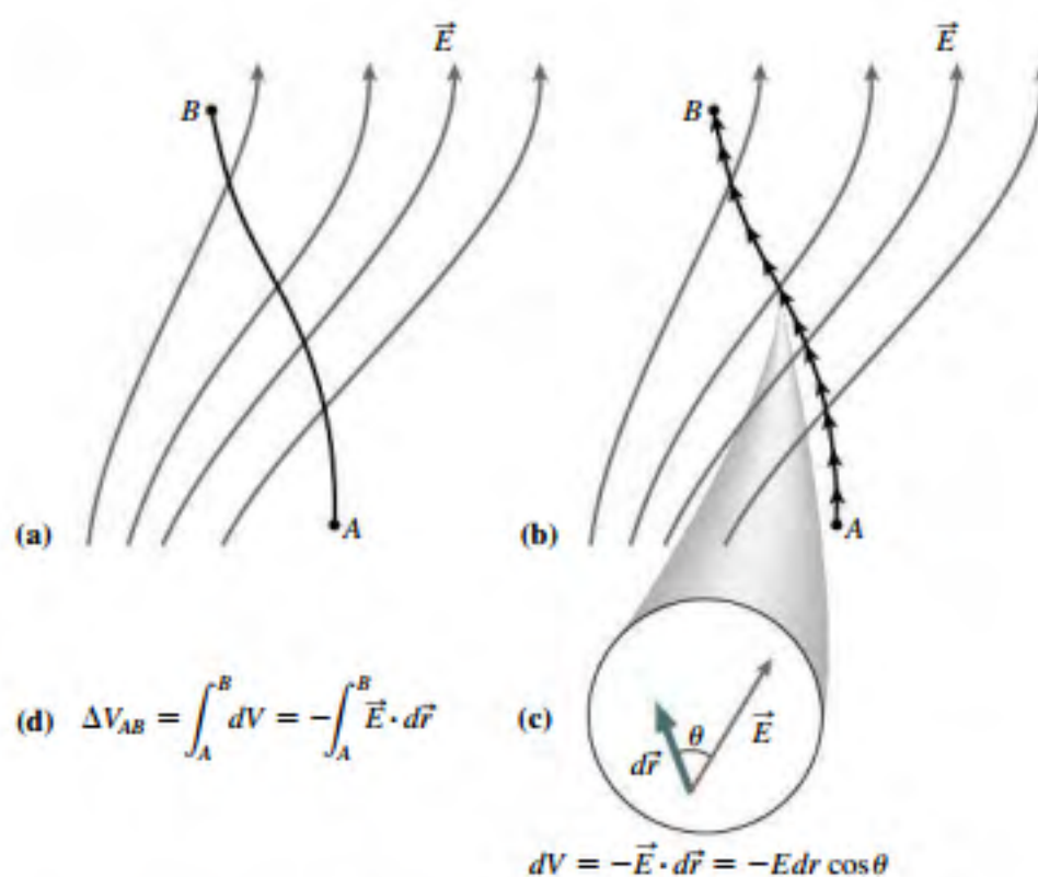
FIGURE 22.5 (a) A path from A to B traverses an electric field \vec{E} . (b) To find the potential difference \Delta V_{AB} , we first divide the path into infinitesimal segments d\vec{r} . (c) The potential difference dV across one such segment is dV = -\vec{E} \cdot d\vec{r} . (d) Adding—that is, integrating—all the dV s along the path gives the expression for \Delta V_{AB} .
