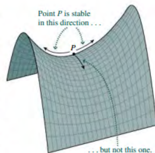
FIGURE 12.10 Equilibrium on a saddle-shaped potential-energy curve.
