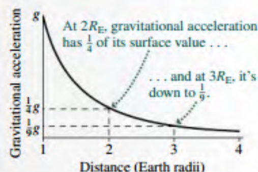
FIGURE 8.3 Meaning of the inverse-square law.
