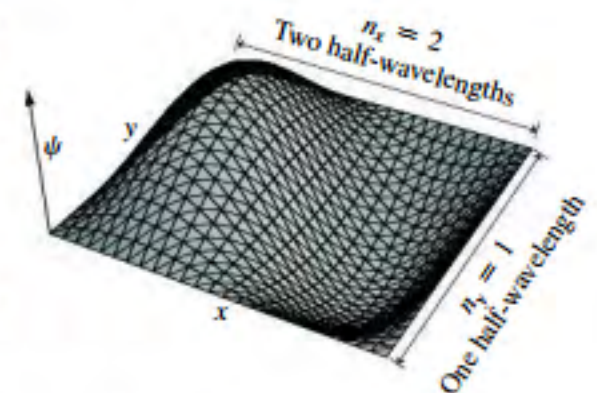
FIGURE 35.16 One possible wave function for a particle confined to a square region in two dimensions. This function is \psi(x, y) = \sin(n_x \pi x/L) \sin(n_y \pi y/L) , with n_x = 2 and n_y = 1 .
