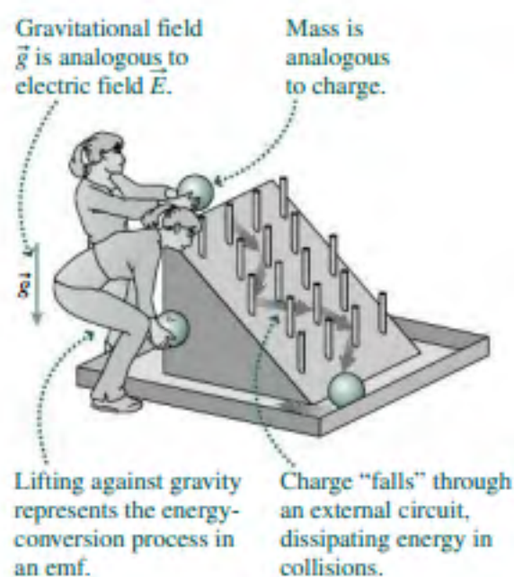
FIGURE 25.2 Gravitational analog for emf.
