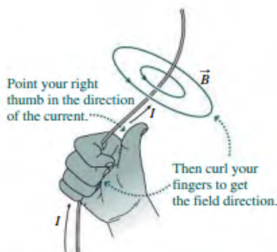
FIGURE 26.16 Magnetic field lines generally encircle a current, with direction given by the right-hand rule.
