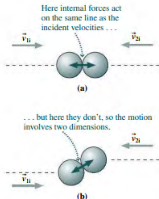
FIGURE 9.16 Only a head-on collision is one-dimensional.
