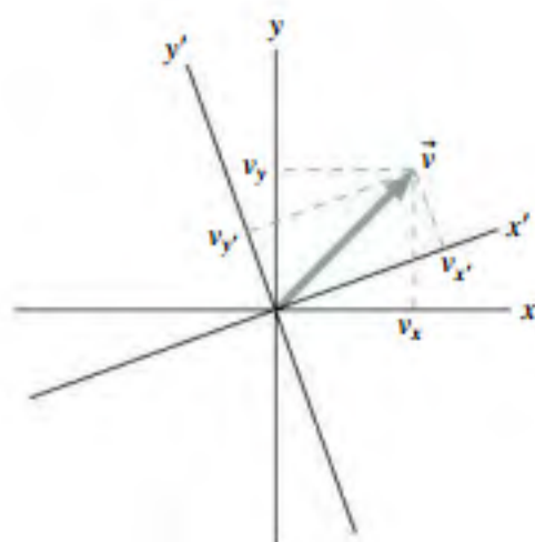
FIGURE 33.18 Although the x - and y -components of an ordinary vector depend on the choice of coordinate system, the magnitude of the vector does not.
