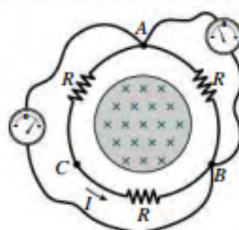
FIGURE 27.31 The work done to move charge in an induced electric field isn't path independent, so the induced field isn't conservative.
