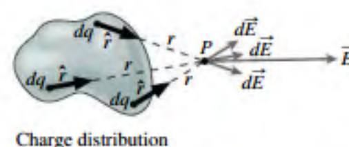
FIGURE 20.15 The electric field at P is the vector sum of the fields d\vec{E} arising from the individual charge elements dq , each calculated using the appropriate distance r and unit vector \hat{r} .
