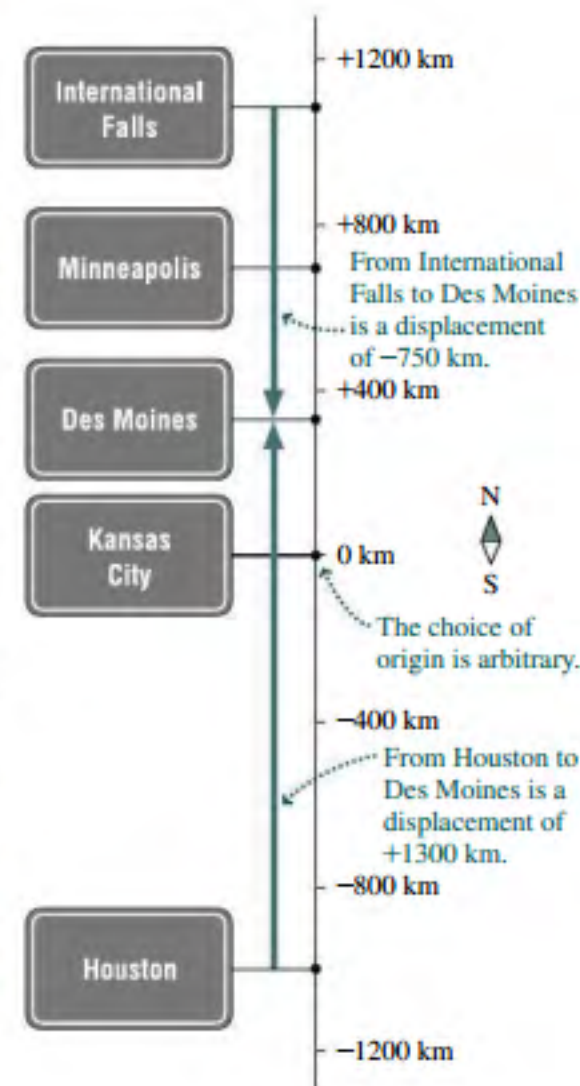
FIGURE 2.2 Describing motion in the central United States.
