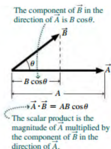
FIGURE 6.6 Geometric interpretation of the scalar product.
