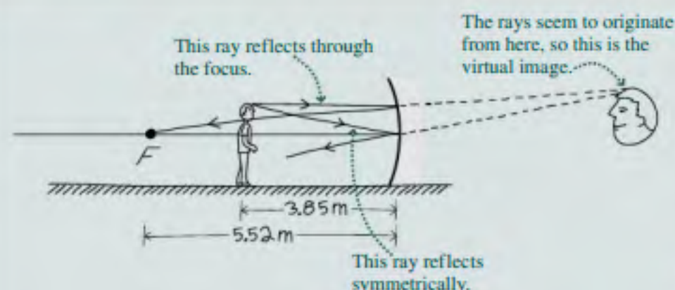
FIGURE 31.12 Sketch for Example 31.1, showing two rays that locate the virtual image of the technician's head.
