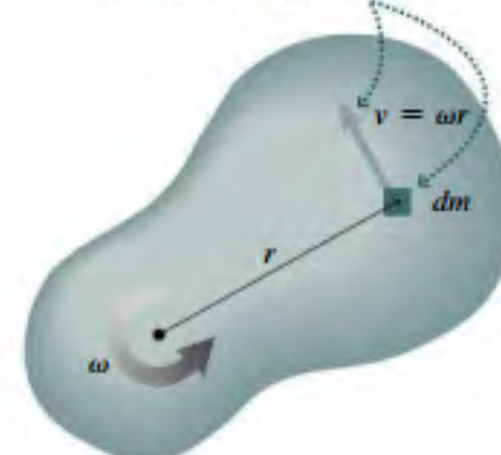
FIGURE 10.21 Kinetic energy of a mass element.
