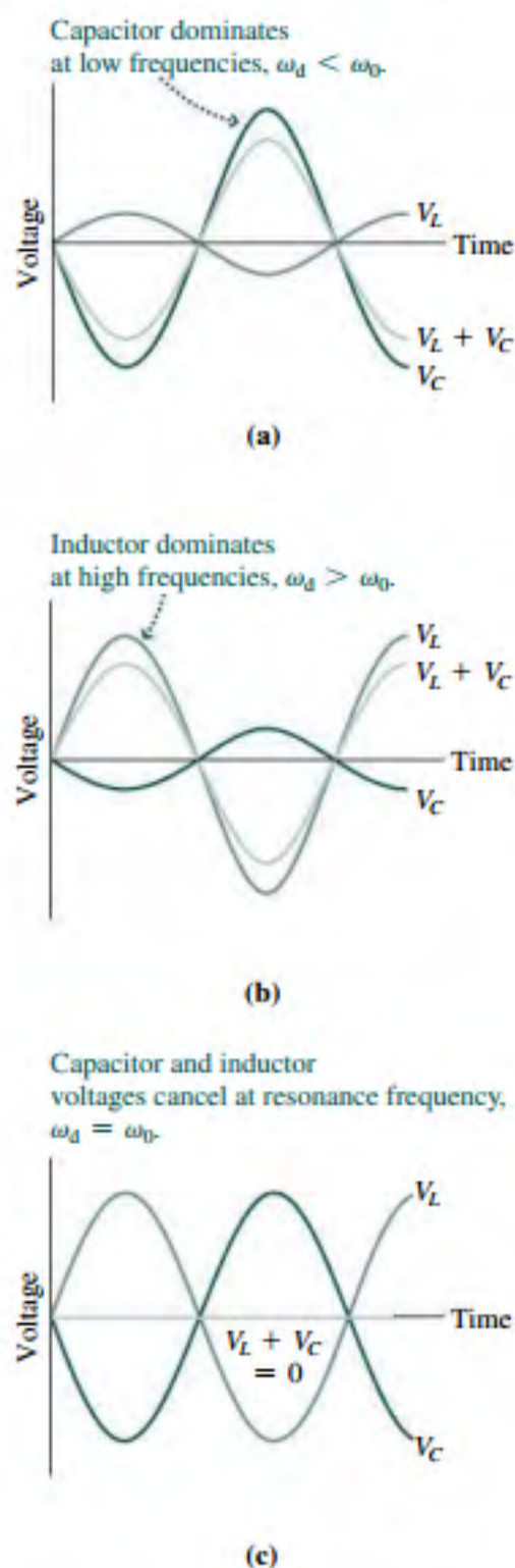
FIGURE 28.15 Capacitor and inductor voltages are always 180^\circ out of phase, but their relative magnitudes vary with frequency.
