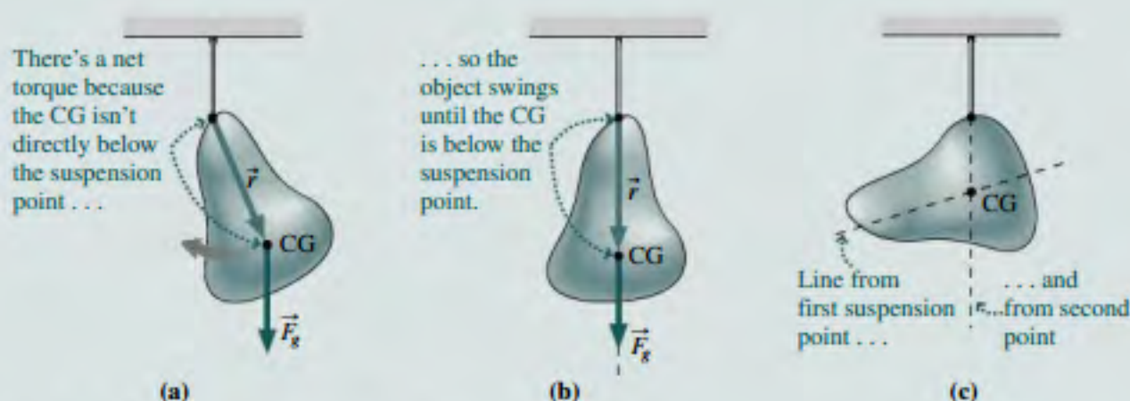
FIGURE 12.3 Finding the center of gravity.
