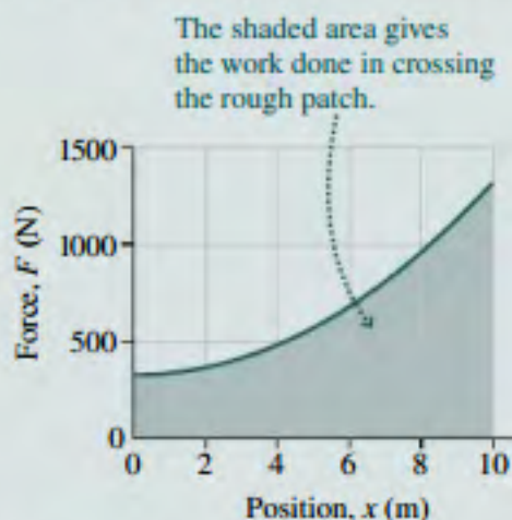
FIGURE 6.13 Force versus position for Example 6.5.
