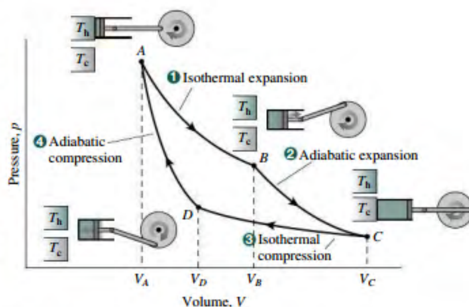
FIGURE 19.5 A pV diagram for the Carnot engine.
