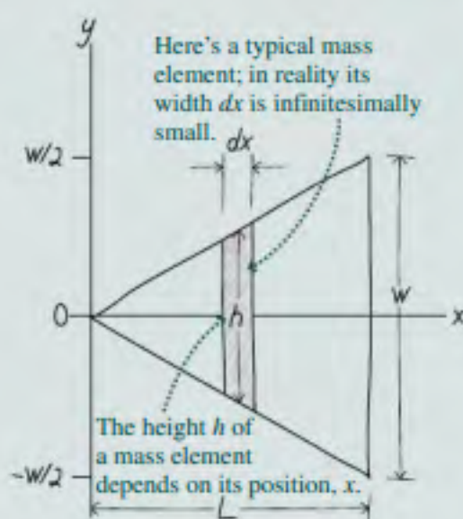
FIGURE 9.4 Our sketch of the supersonic aircraft wing.
