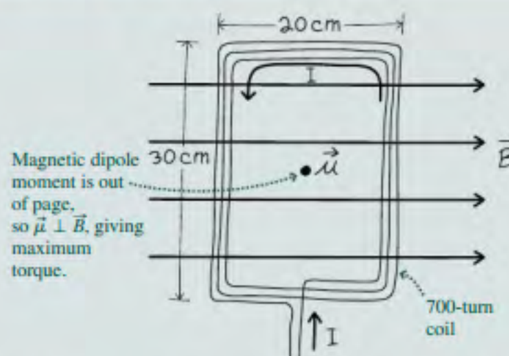
FIGURE 26.24 Loop for the motor of Example 26.5, shown in the position of maximum torque.
