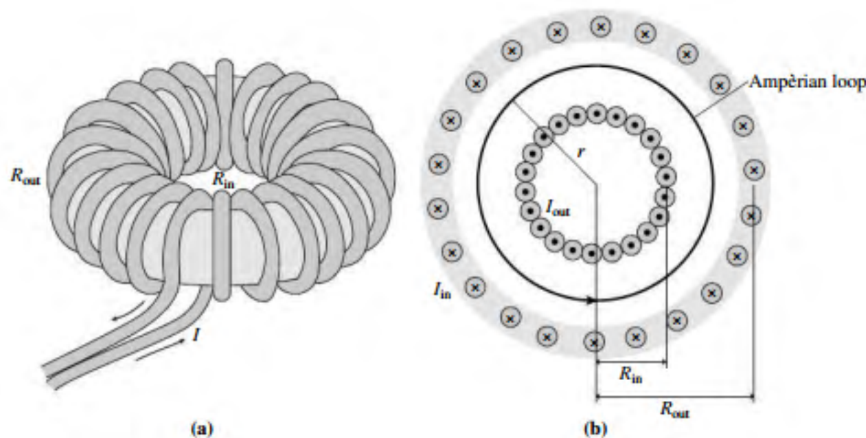
FIGURE 26.53 Diagram of (a) a toroidal coil and (b) a cross section of the coil (Passage Problems 88–91)
