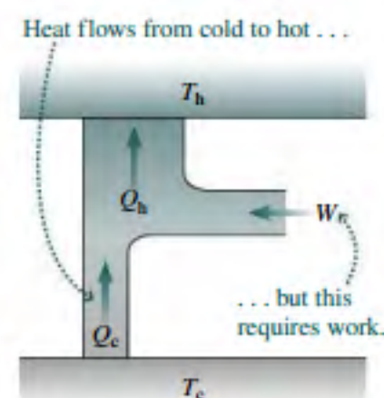
FIGURE 19.6 Energy-flow diagram for a real refrigerator.
