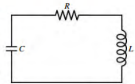
FIGURE 28.12 An RLC circuit.
