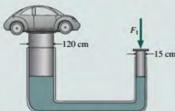
FIGURE 15.6 A hydraulic lift.
