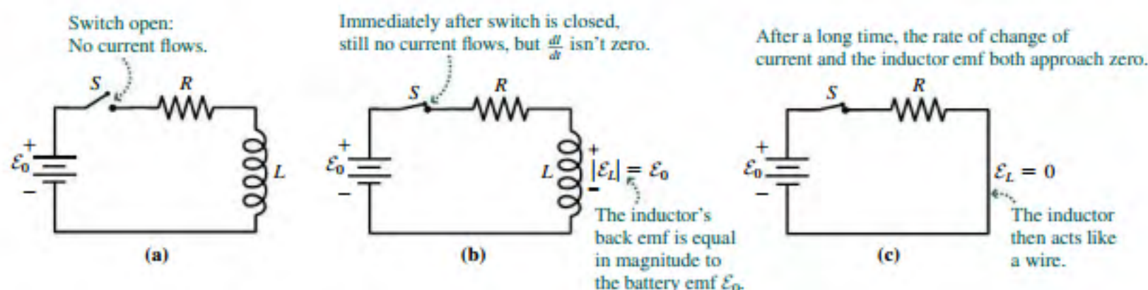
FIGURE 27.23 An RL circuit at three times.
