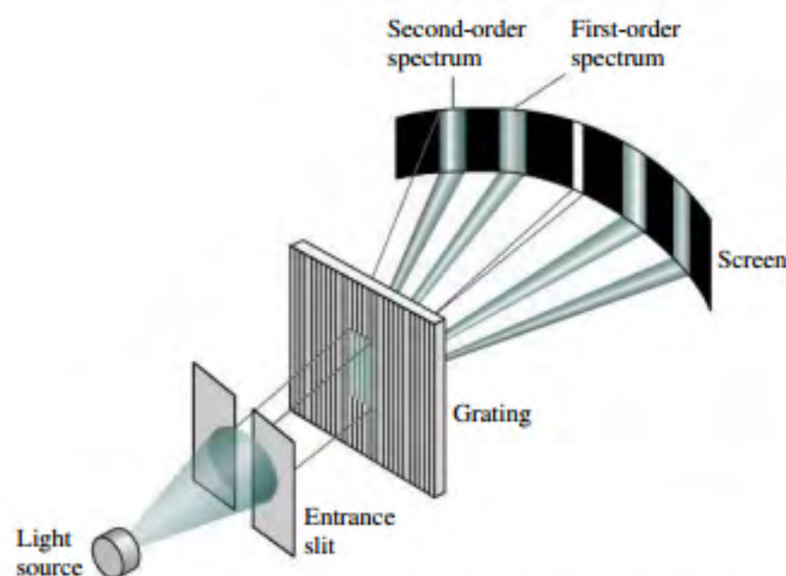
FIGURE 32.9 Essential elements of a grating spectrometer. An electronic detector normally replaces the screen.
