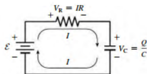
FIGURE 25.20 Voltage changes in a charging RC circuit.
