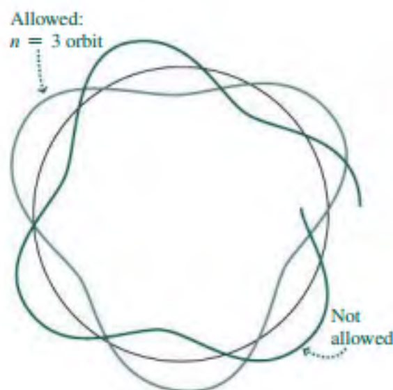
FIGURE 34.11 The allowed electron orbits in the Bohr atom are those that can fit an integral number of de Broglie wavelengths around the circular Bohr orbit.
