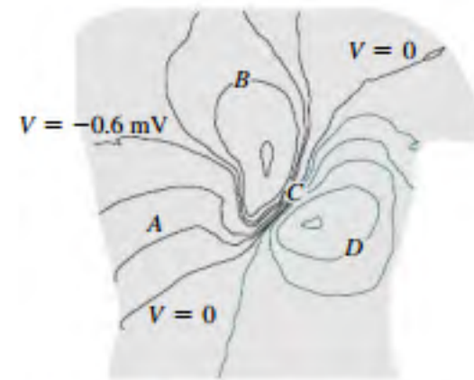
FIGURE 22.26 Equipotentials on a human torso (Passage Problems 84–87)
