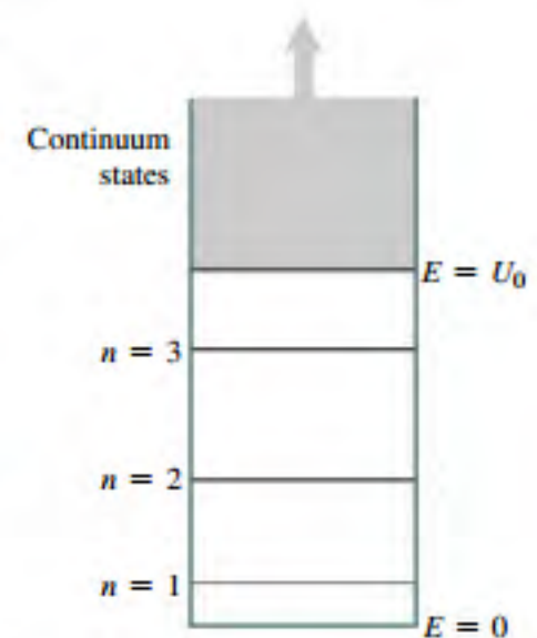
FIGURE 35.15 Energy-level diagram for a finite square well shows discrete bound states and a continuum of unbound states.
