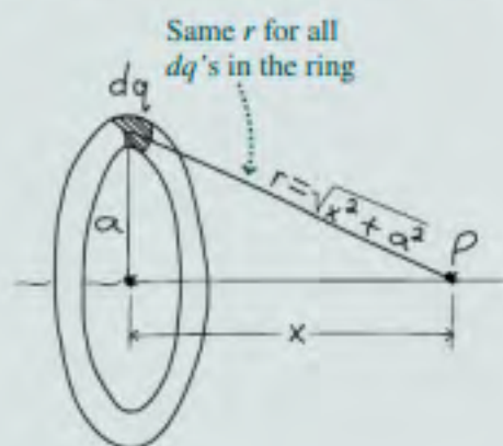
FIGURE 22.12 A charged ring.
