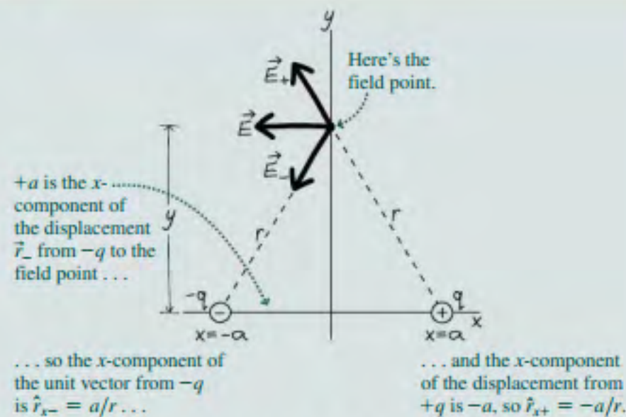
FIGURE 20.13 Finding the field of an electric dipole.
