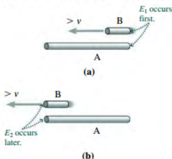
FIGURE 33.11 The passing rods viewed in a reference frame S' at rest with respect to rod A.
