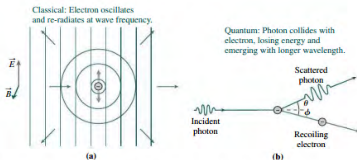
FIGURE 34.8 Classical and quantum descriptions of the interaction between electromagnetic waves and free electrons.
