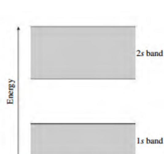
FIGURE 37.14 Energy-level diagram for the equilibrium separation of Fig. 37.13c.
