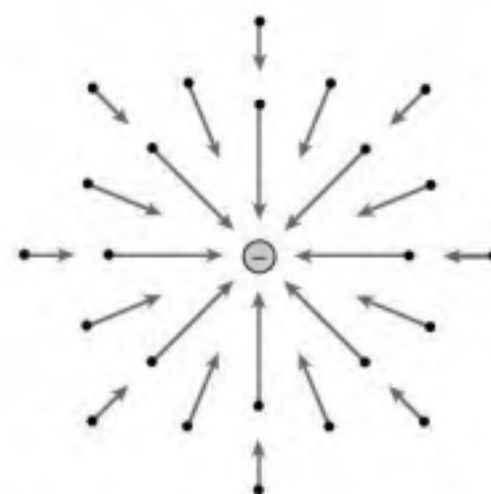
FIGURE 20.9 Field vectors for a negative point charge.
