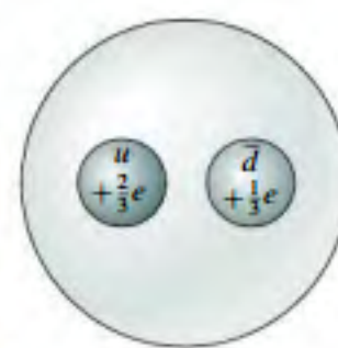
FIGURE 39.5 Mesons consist of a quark and an antiquark. The meson here is the \pi^+ , made from an up quark and a down antiquark.
