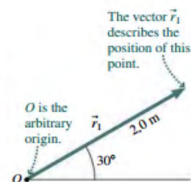
FIGURE 3.1 A position vector \vec{r}_1 .
