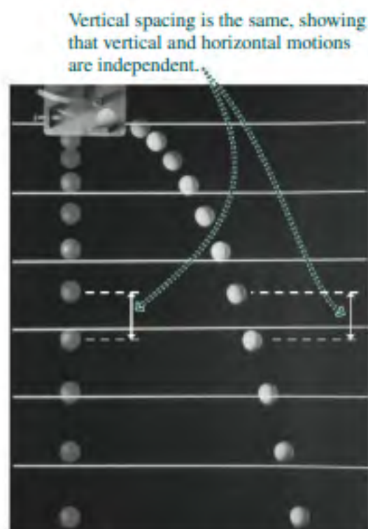
FIGURE 3.11 Two marbles, one dropped and the other projected horizontally.
