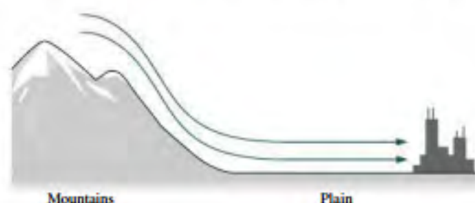
FIGURE 18.24 Chinooks (Passage Problems 80–83)
