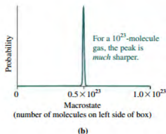
FIGURE 19.21 Probability distributions for a gas of (a) 100 molecules and (b) 10^{23} molecules.
