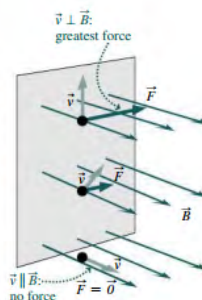
FIGURE 26.2 The magnetic force on a charged particle is perpendicular to both the particle's velocity \vec{v} and the magnetic field \vec{B} . The force shown here has the direction appropriate to a positively charged particle.
