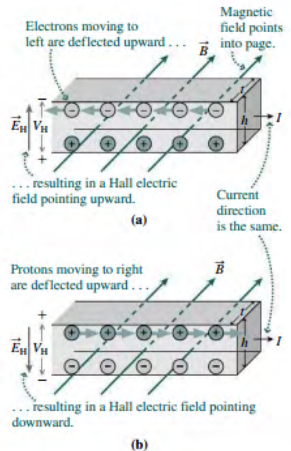
FIGURE 26.14 The Hall electric field \vec{E}_H and Hall potential V_H arise from the magnetic deflection of charge carriers. In both (a) and (b) the current is to the right, carried in (a) by negative charge moving to the left and in (b) by positive charge moving to the right.
