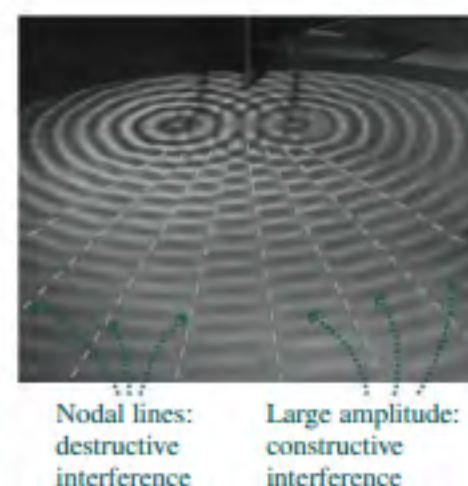
FIGURE 14.21 Water waves from two sources interfere to produce regions of low and high amplitude.
