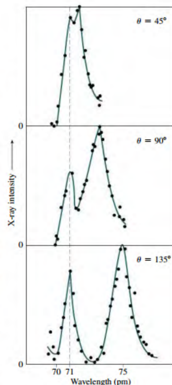
FIGURE 34.9 Compton's results for scattering of X-rays with \lambda = 71 \text{ pm} (indicated by the vertical dashed line). Right-hand peak shows the wavelength shift of the Compton effect. The unshifted left-hand peak is from photons scattering off tightly bound atomic electrons, which don't absorb significant energy. Solid curves are theoretical predictions.
