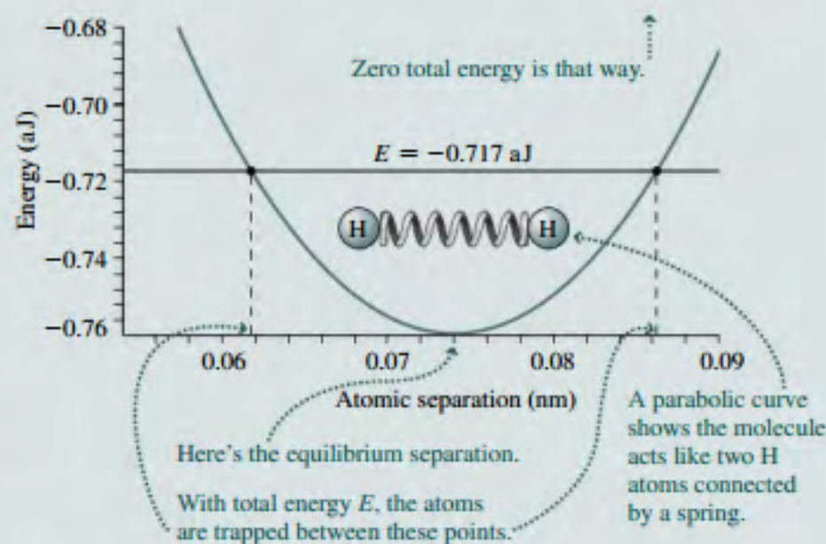
FIGURE 7.12 Analyzing the hydrogen molecule.
