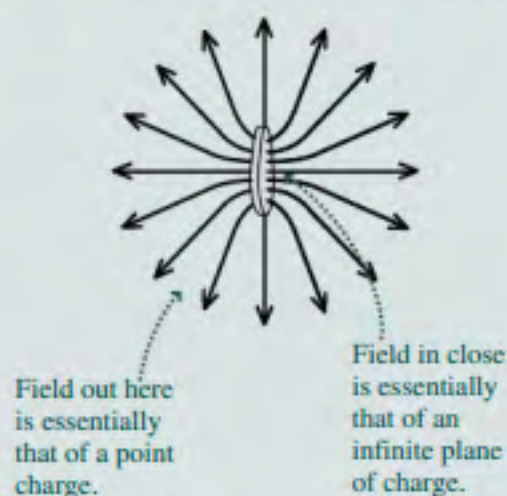
FIGURE 21.22 The electric field of a charged disk.
