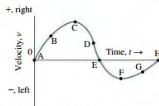
FIGURE 2.16 The tiger's velocity (Passage Problems 98–102.)
