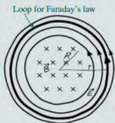
FIGURE 27.30 Cross section of a solenoid whose magnetic field points into the page and is increasing in strength. Field lines of the induced electric field are circles concentric with the solenoid axis.
