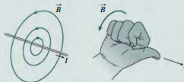
FIGURE 26.19 Magnetic field lines encircle a straight wire, with their direction given by the right-hand rule.
