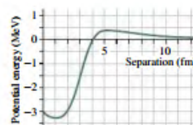
FIGURE 7.24 Potential energy for two deuterons (Passage Problems 70–73)
