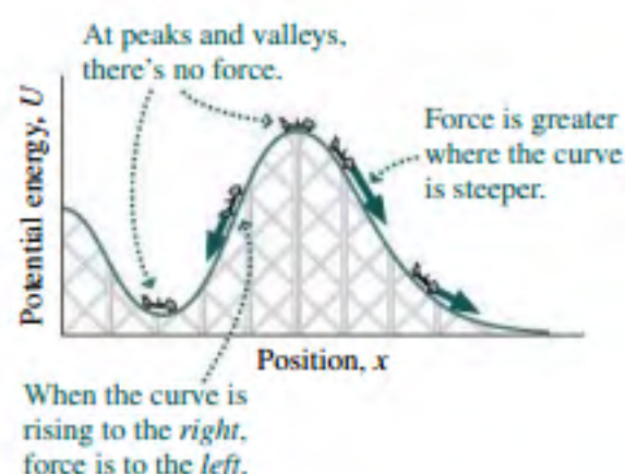
FIGURE 7.13 Force depends on the slope of the potential-energy curve.
