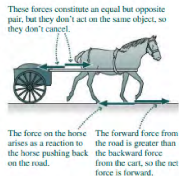
FIGURE 4.14 The horse-and-cart dilemma: The horse pulls on the cart, and the cart pulls back on the horse with a force of equal magnitude. So how can the pair ever get moving? No problem: The net force on the horse involves forces from different third-law pairs. Their magnitudes aren't equal, and the horse experiences a net force in the forward direction.
