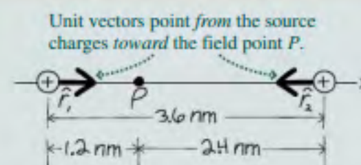
FIGURE 20.10 Finding the electric field at P .
