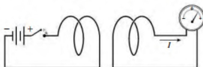
FIGURE 27.4 A current is also induced when the current in an adjacent circuit changes, here as the switch is opened or closed.
