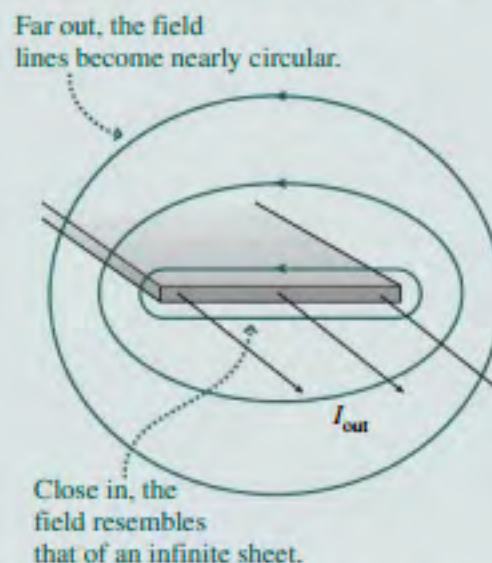
FIGURE 26.33 Field of a finite-width current sheet.
