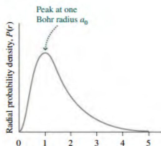
FIGURE 36.3 Radial probability density for the hydrogen ground state.
