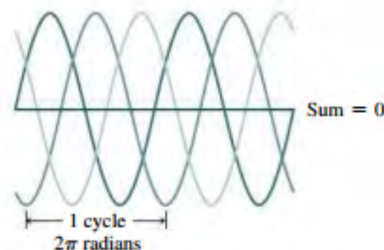
FIGURE 32.7 Waves from three slits must be out of phase by one-third of a cycle in order to interfere destructively.
