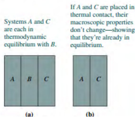
FIGURE 16.1 The zeroth law of thermodynamics.
