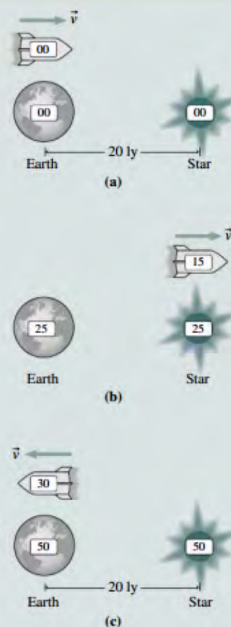
FIGURE 33.8 The twin's journey, drawn from the viewpoint of the Earth–star reference frame. Clock readings are in years, corresponding to Example 33.2.
