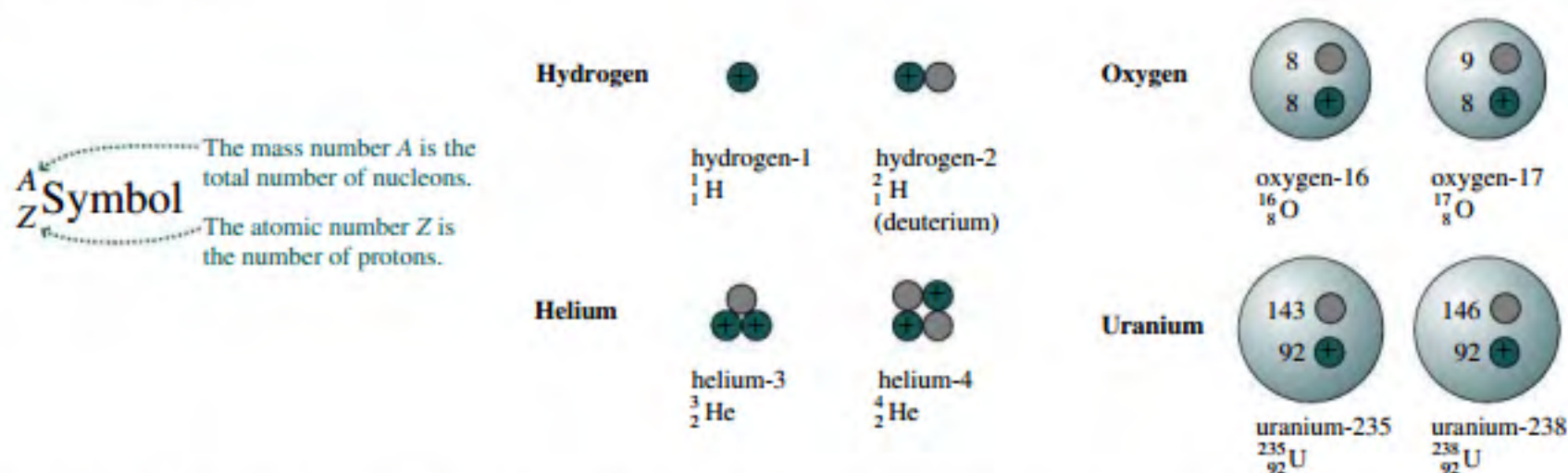
FIGURE 38.1 Isotopes of a given element have the same number of protons but different numbers of neutrons.
