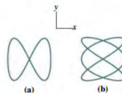
FIGURE 13.18 Complex paths resulting from different frequencies in different directions. Can you determine the frequency ratios?
