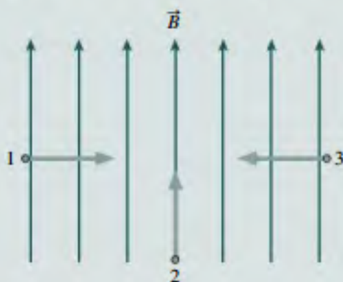
FIGURE 26.4 What's the magnetic force on each proton?
