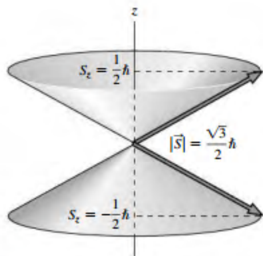
FIGURE 36.8 Space quantization of electron spin.
