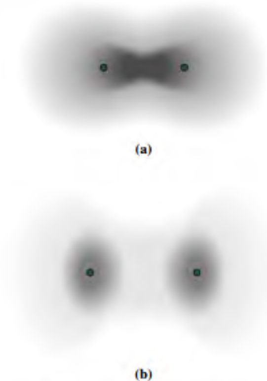
FIGURE 37.6 Electron probability densities for (a) the ground state and (b) the first excited state of hydrogen. Note that the nuclei are farther apart in the excited state.
