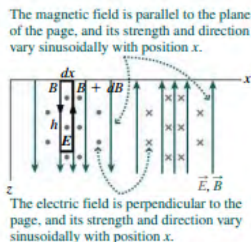
FIGURE 29.5 View of Fig. 29.3b in the x - z plane, with a rectangular loop for evaluating the line integral in Ampère's law.
