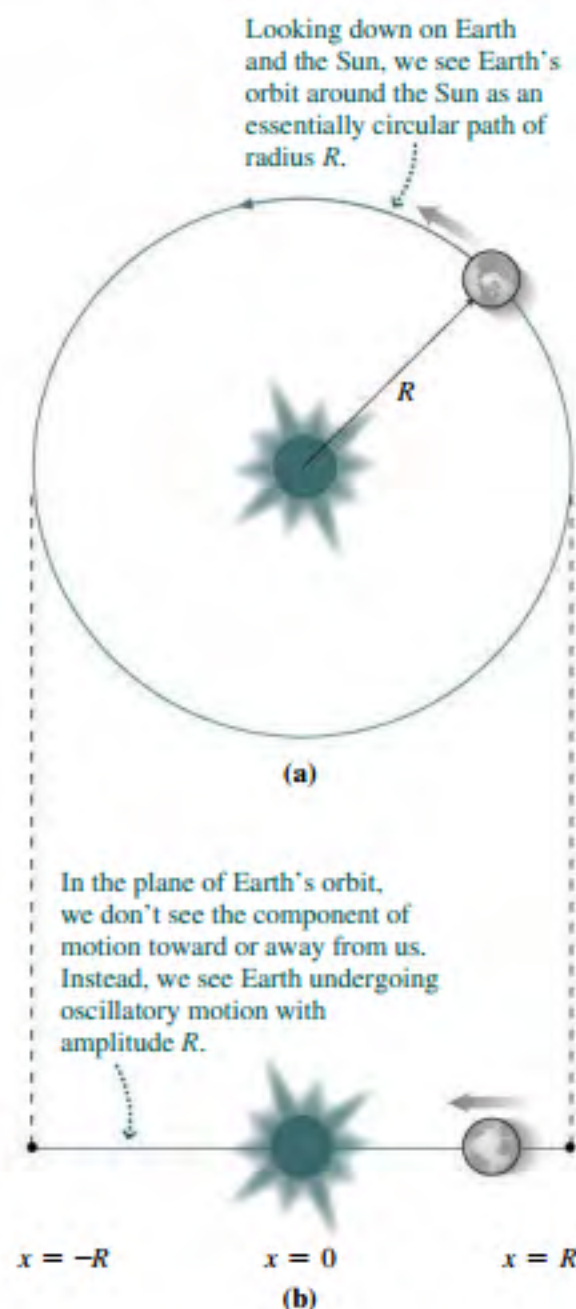
FIGURE 13.16 Two views of Earth's orbital motion.
