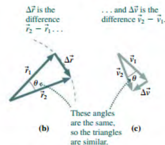
FIGURE 3.22 Position and velocity vectors for two nearby points on the circular path.
