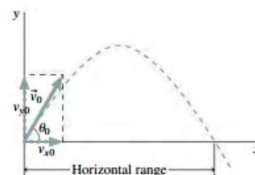
FIGURE 3.17 Parabolic trajectory of a projectile.
