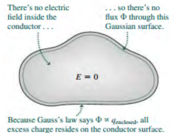
FIGURE 21.24 Gauss's law implies that any net charge resides on the surface of a conductor in electrostatic equilibrium.
