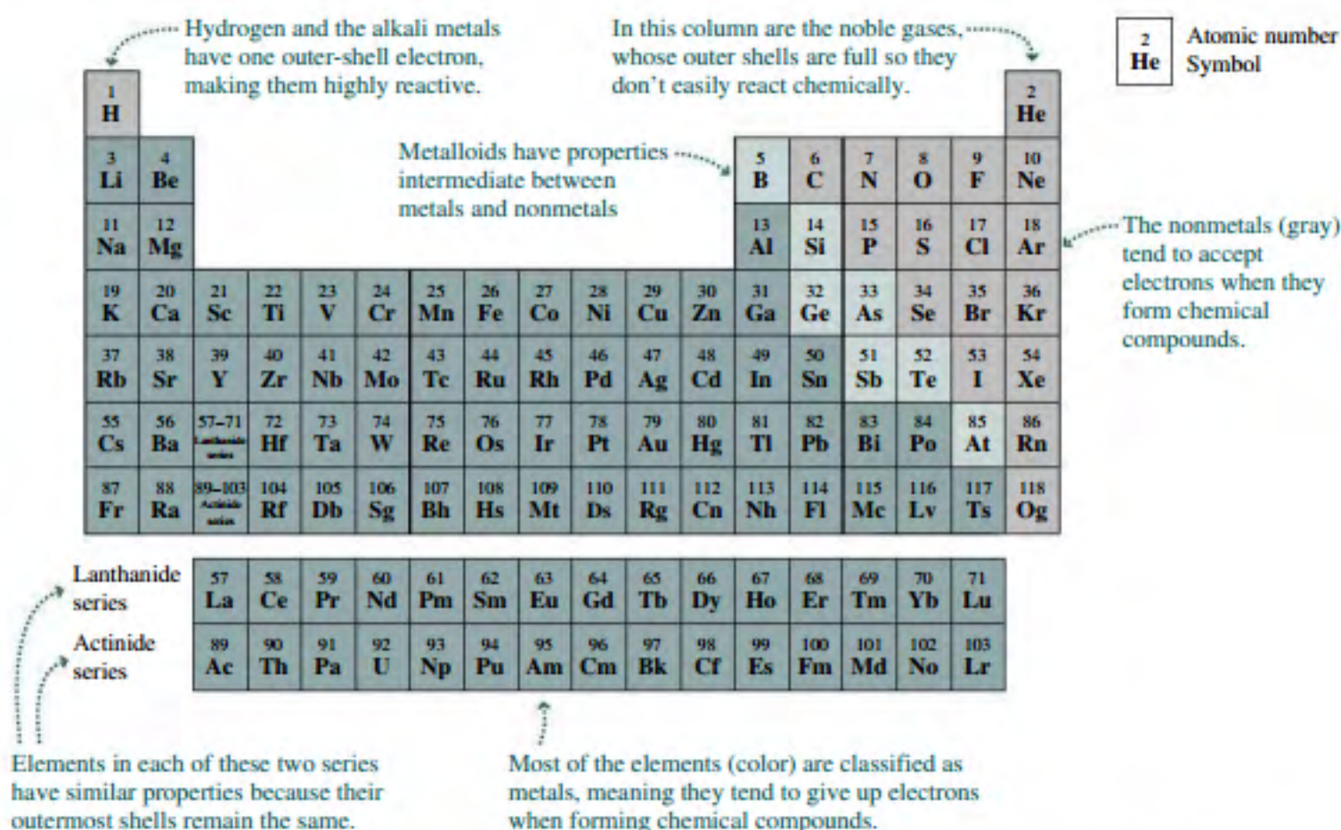
FIGURE 36.15 The periodic table. A larger version, with atomic weights, is inside the back cover; the names of the elements are in Appendix D.
