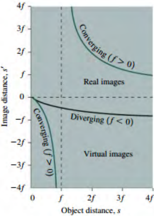
FIGURE 31.20 Image distance versus object distance for lenses.
